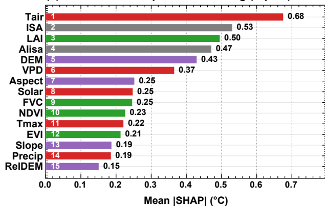
(a) Global driver-importance ranking (top 15)
