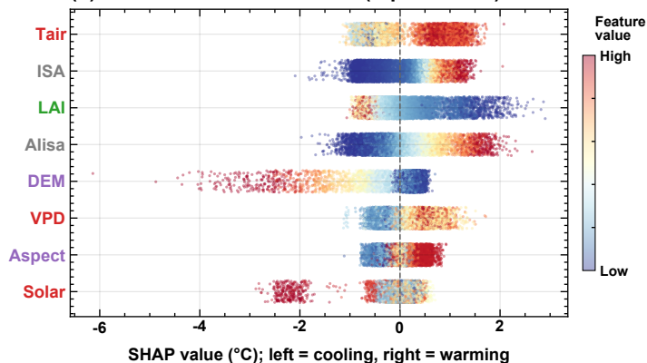
(b) Per-cell SHAP distribution (top 8 drivers)
