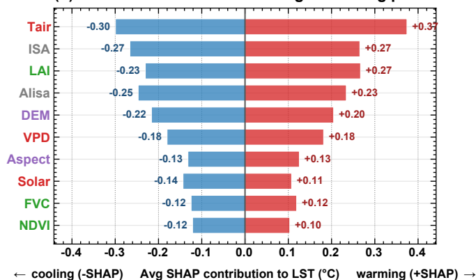
(d) Bidirectional effects: warming vs cooling per driver
