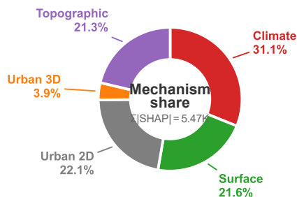
(c) Driver-category share of total |SHAP|
