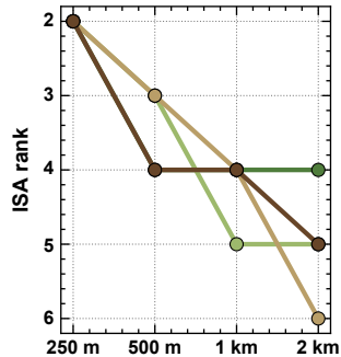
(c) ISA (urban 2D)
