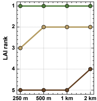
(b) LAI (vegetation)
