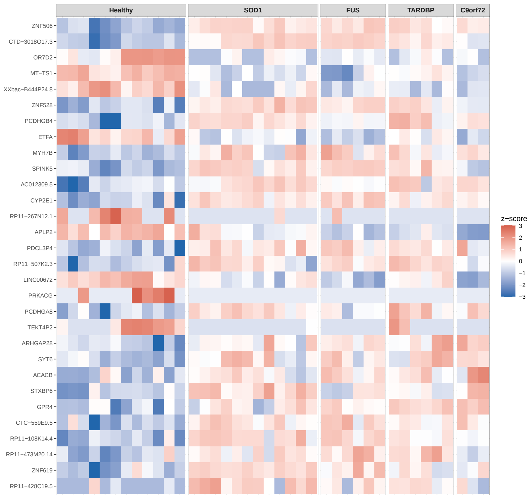
Top 30 elastic-net selected genes (iMN day 28)
