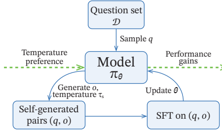
(b) Workflow of SePT.
