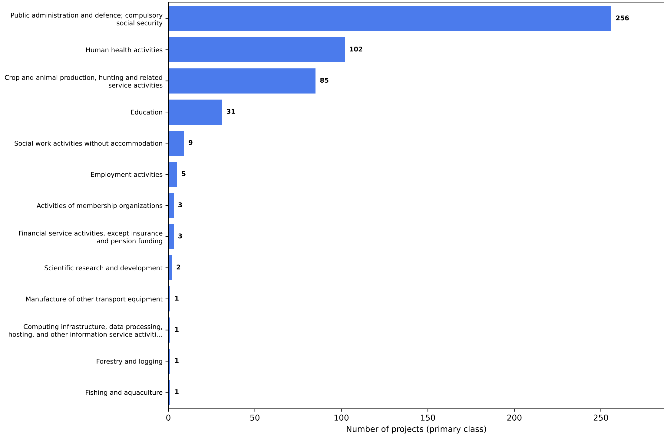
ihsn — Histogram of primary ISIC classes
