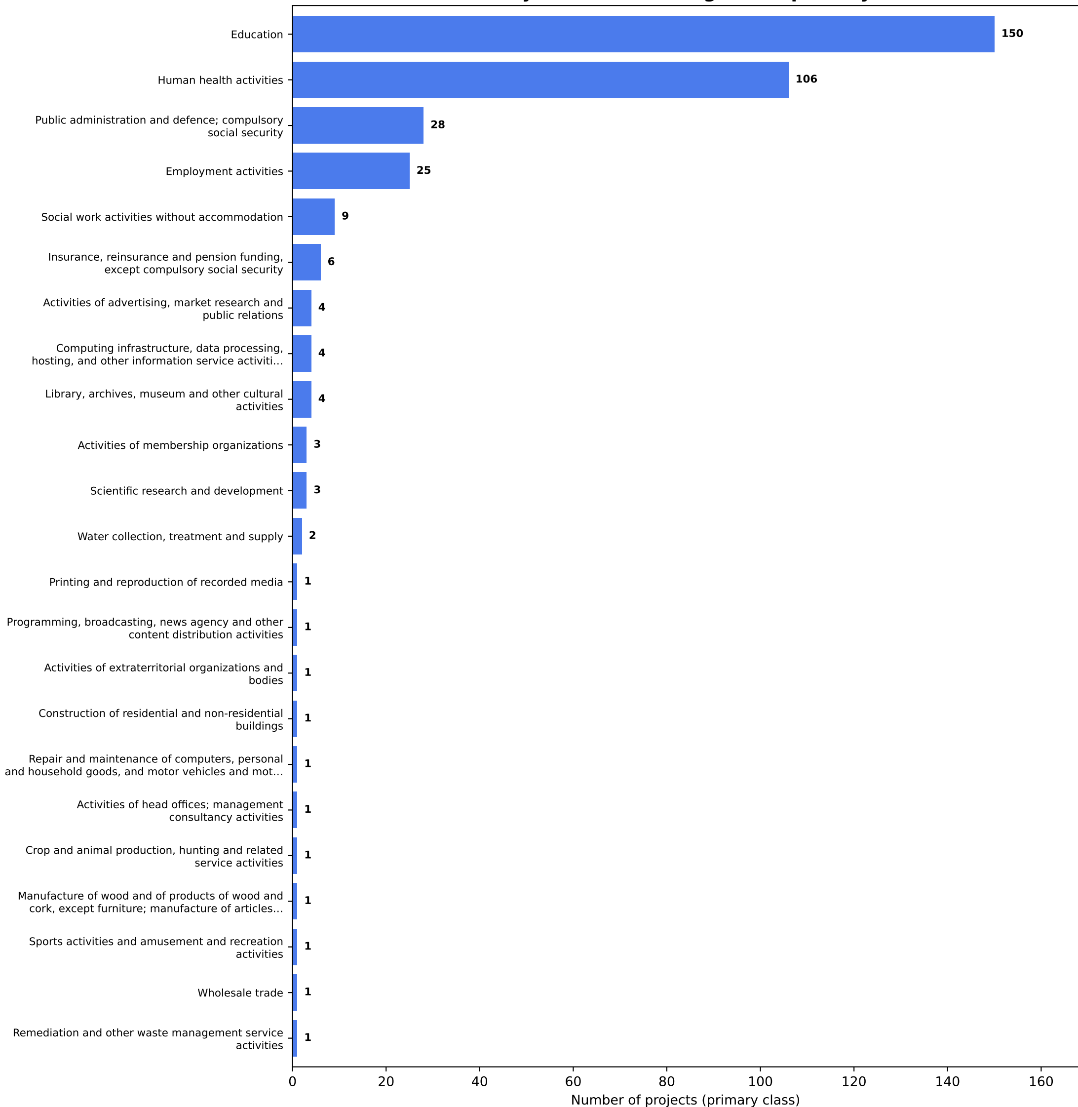
harvard-murray-archive — Histogram of primary ISIC classes
