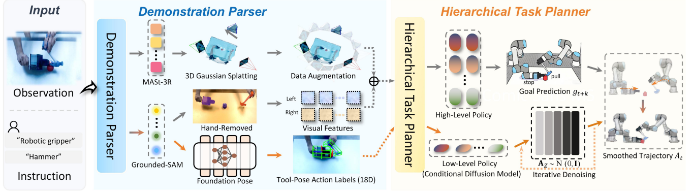
Fig. 2. The technical architecture of the TAC. TAC takes visual observations and instructions as inputs. The demonstration parser uses MAST-3R and Gaussian splatting for 3D reconstruction, FoundationPose for pose estimation, and Grounded-SAM for morphological decoupling, automatically converting human videos into structured training data. The final training samples include hand-removed tool-centric observations and the corresponding 18D tool-pose action labels. During deployment, the hierarchical planner first predicts short-term coordinated goals, and the low-level diffusion policy then generates specific, coordinated bimanual trajectories to execute the task.
