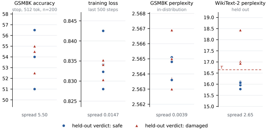
Figure 5: The same eight blockwise runs at 3B under four measurements. Color marks the pre-specified verdict, which is defined on held-out perplexity. Only that panel separates the colors: task accuracy, training loss and in-distribution perplexity interleave the two groups completely. Accuracy is the unified protocol of §4.1; training loss is the mean over the final 500 optimizer steps. The figure under each panel is the spread across the eight runs, in that panel’s units.
