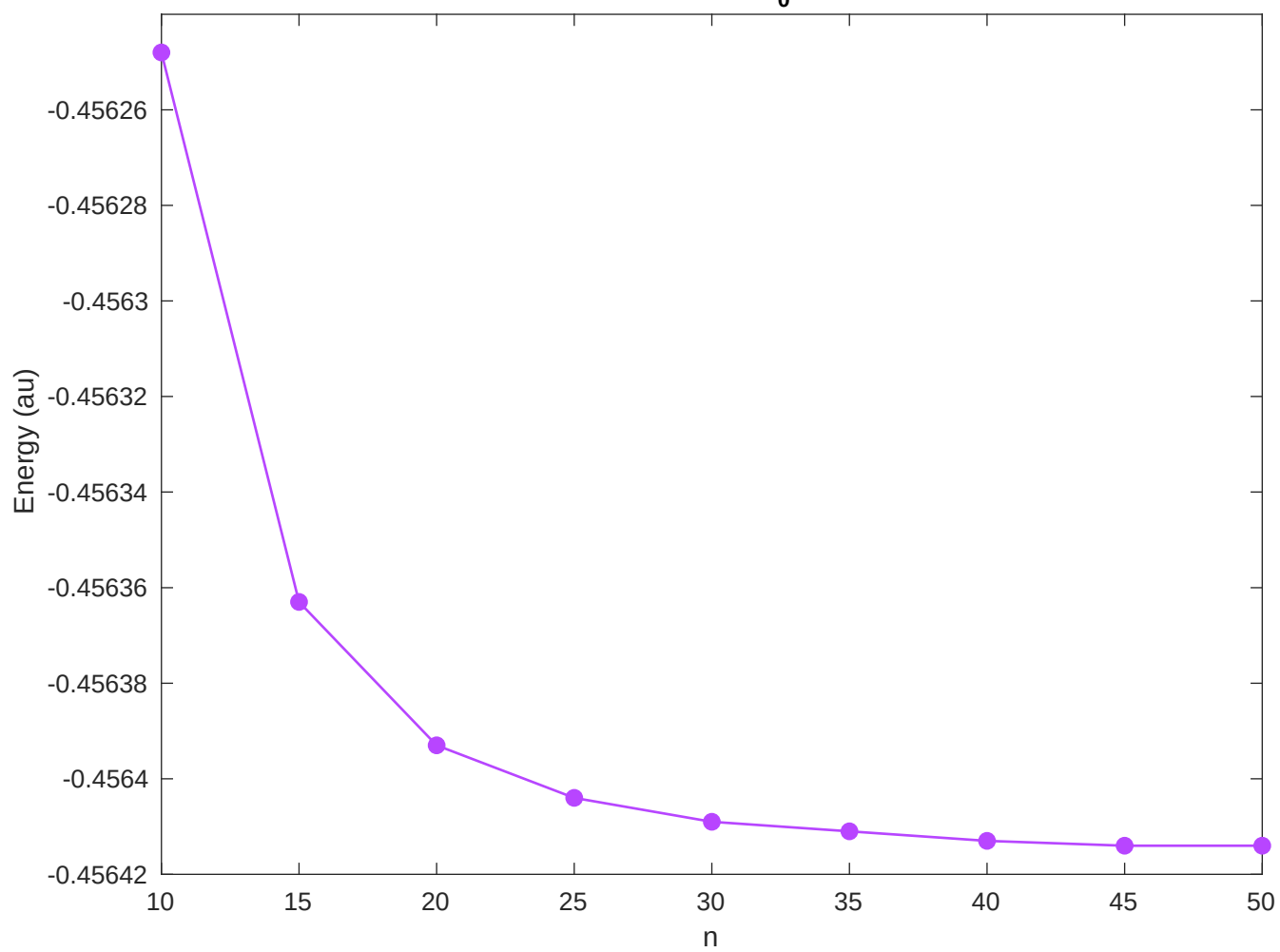
Energy v/s number of plane waves(= 2n+1) a = 10, b = 2, V_0 = 1
