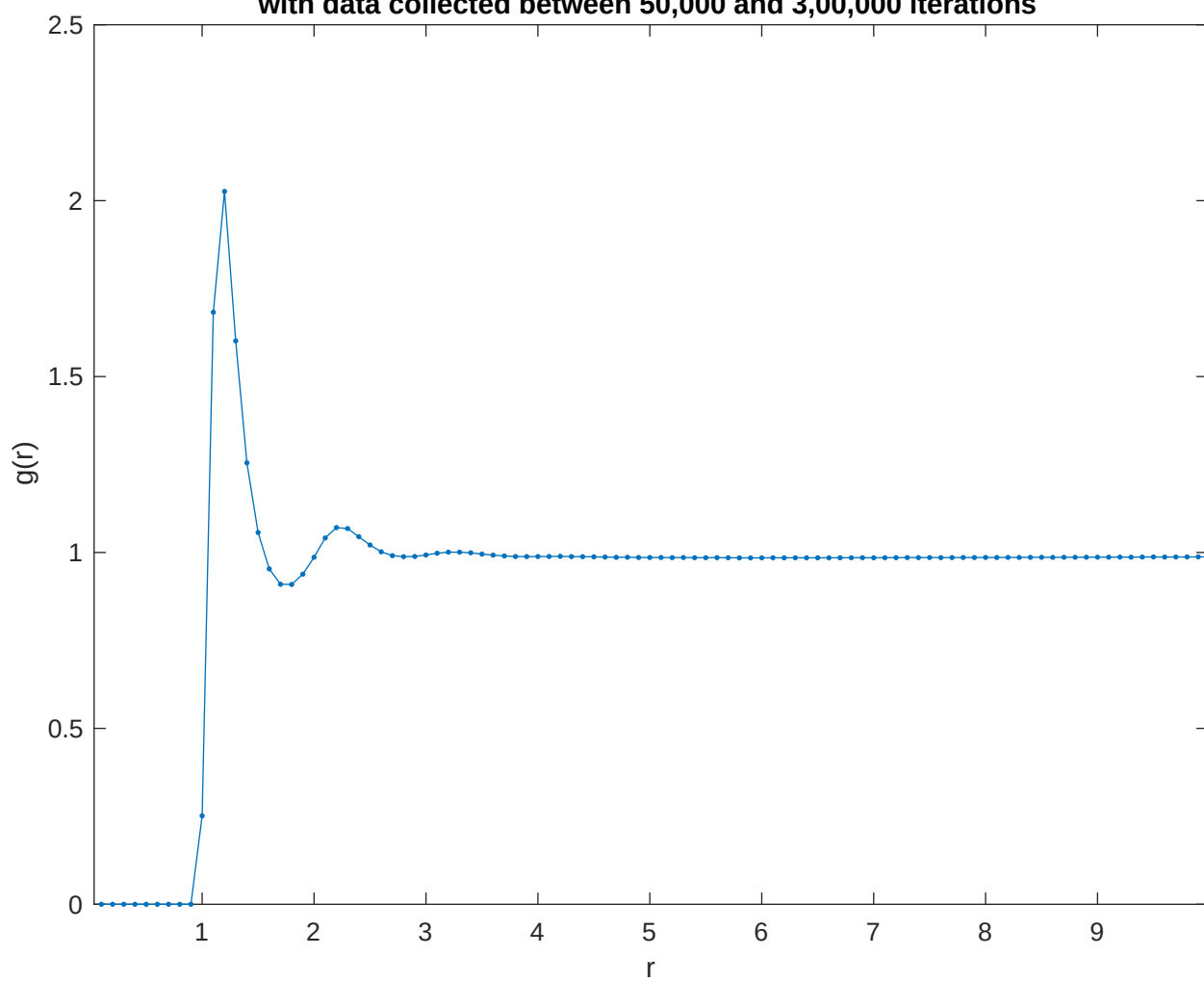
Graph of correlation function with 2400 particles with data collected between 50,000 and 3,00,000 iterations
