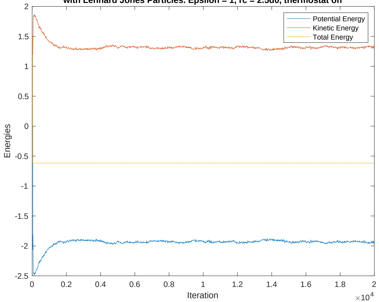
MD simulation with 2197 particles in a 20*20*20 box with dt = 0.005 with Lennard Jones Particles. Epsilon = 1, rc = 2.5d0, thermostat off
