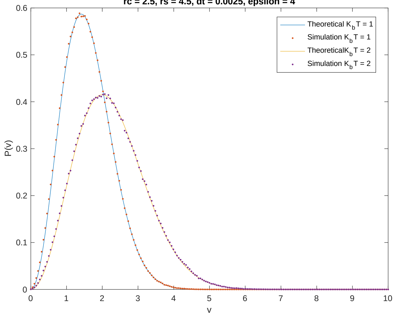
Speed distribution for 1200 particles in a 20*20*20 box at K_b T = 1 rc = 2.5 , rs = 4.5 , dt = 0.0025 , \epsilon = 4
