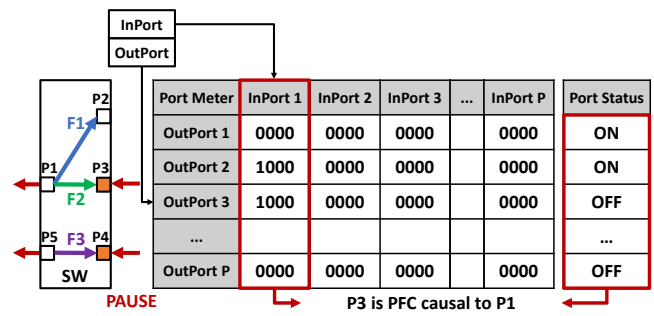
Figure 3: HAWKEYE PFC causality structure.
