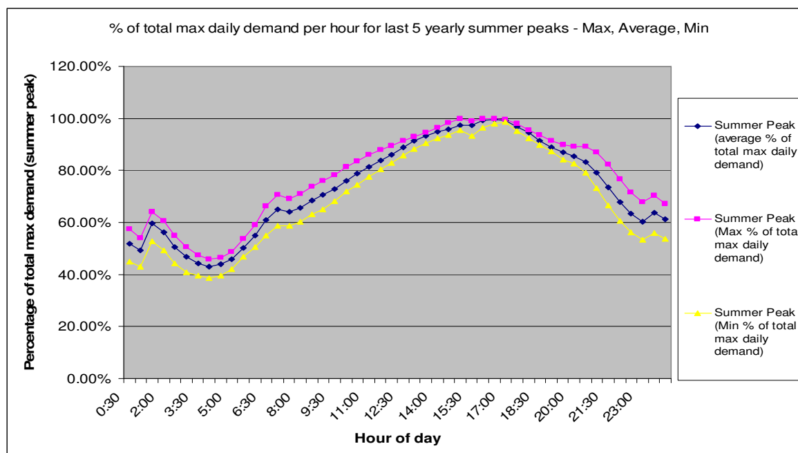
Figure 1.2 Average, Maximum and Minimum Utilisation for the last 5 Peak Summer Days
