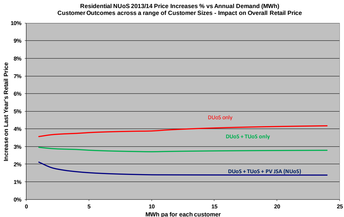
Figure 5 - Low voltage residential Retail price change in 2013/14
