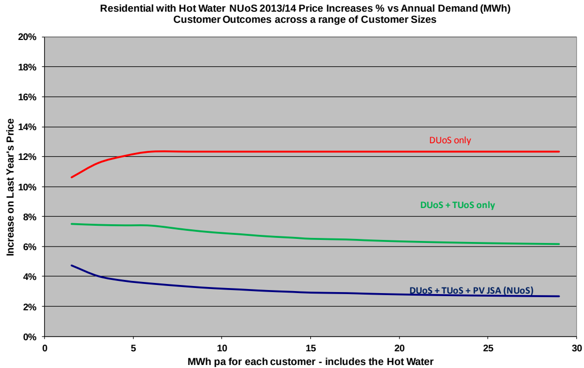
Figure 6 - Low voltage residential + hot water NUoS price change in 2013/14
