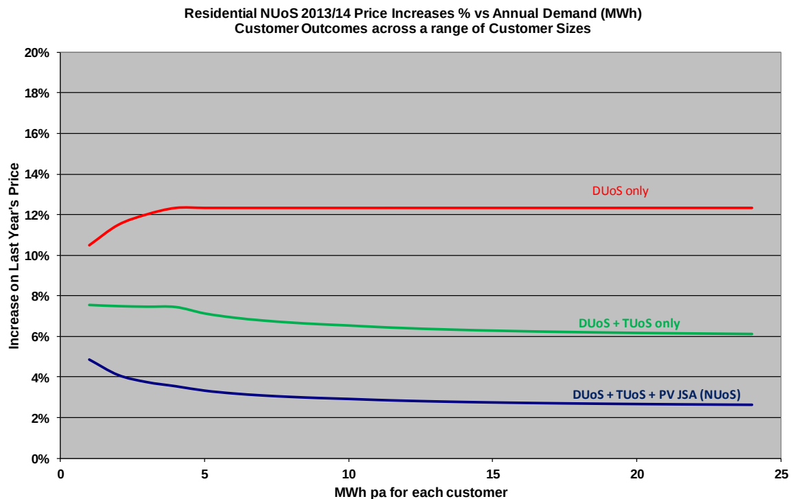
Figure 4 - Low voltage residential NUoS price change in 2013/14
