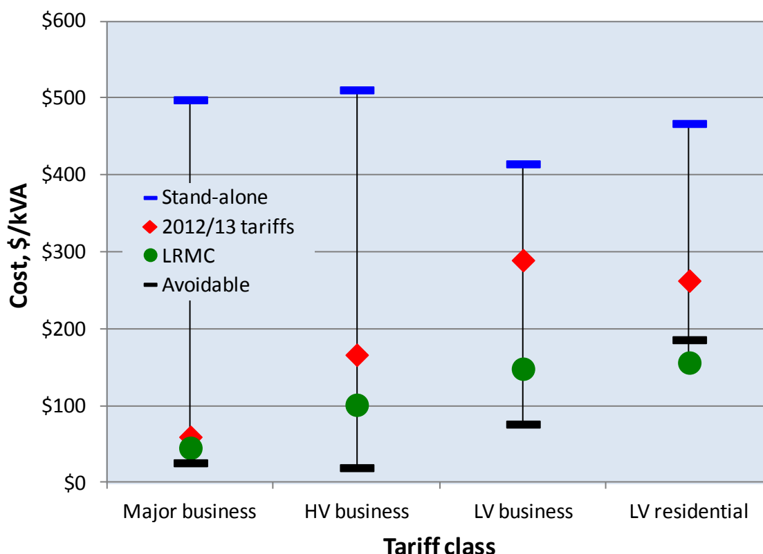
Figure 14 - Cost comparison ($/kVA per annum)
