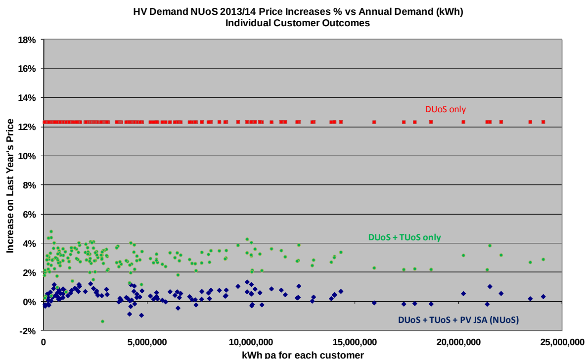
Figure 13 - High voltage business kVA NUoS change vs annual consumption in 2013/14
