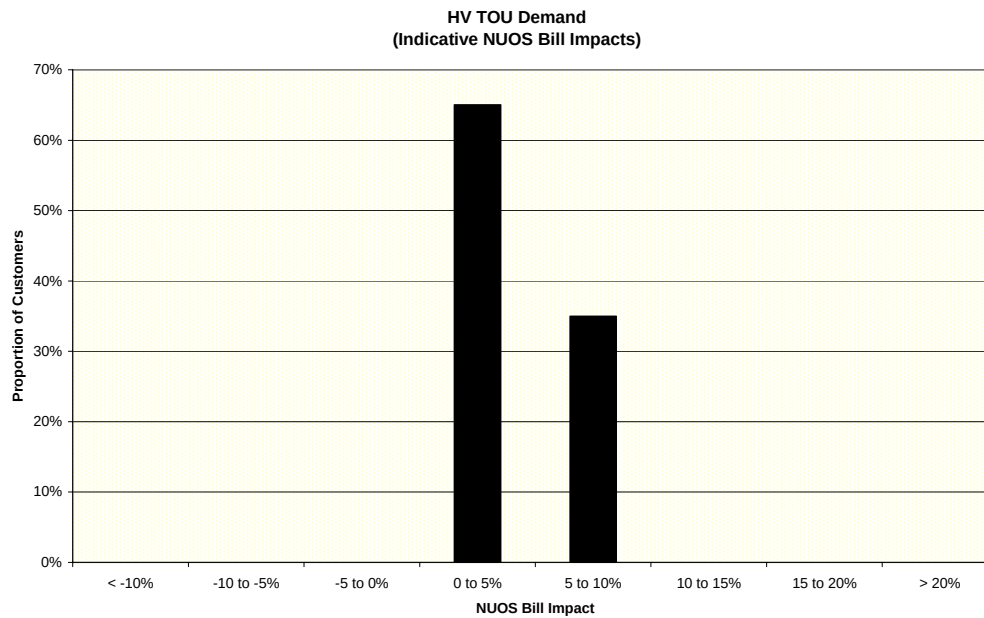
Figure 6-3: Customer Impact (Nominal Terms) – HV TOU Demand Network Tariff
