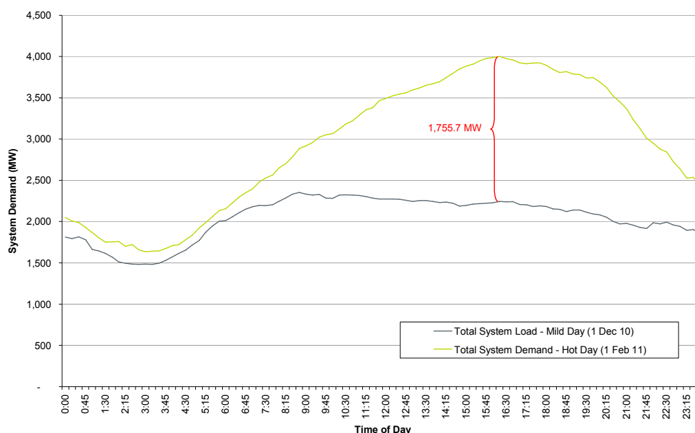
Figure 3.5: Peak demand on an extreme temperature day relative to mild summer day
