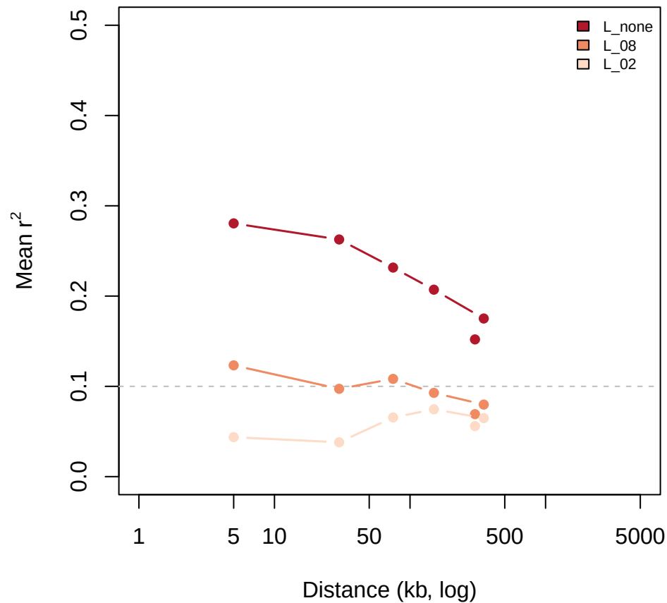
HDRA LD decay (chr1)
