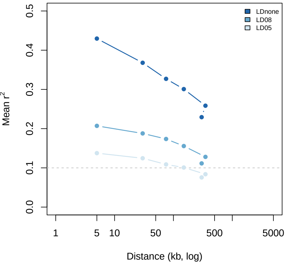
44K LD decay (chr1)
