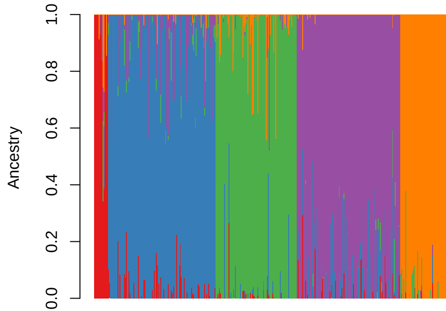
ADMIXTURE K = 5
