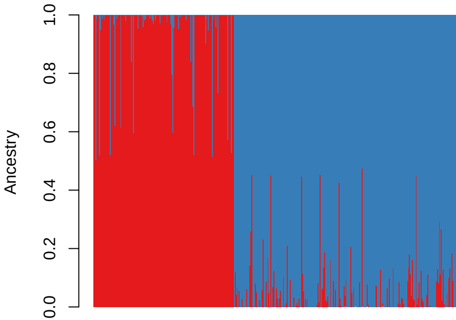
ADMIXTURE K = 2
