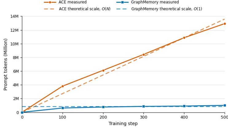
Figure 1: Prompt-token usage at successive training checkpoints for GraphMemory and ACE on FORMULA with Qwen3.8-27B.
