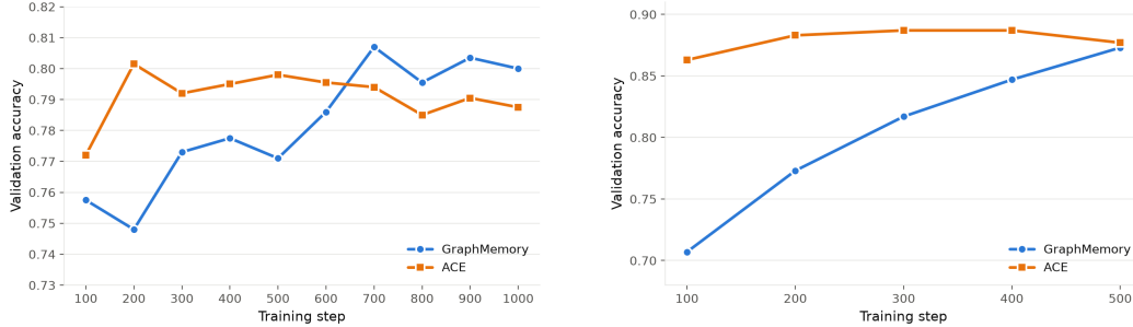
Figure 3: Validation performance of GraphMemory and ACE on Claude across training steps on FiNER (left) and FORMULA (right).
