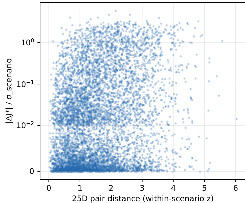
(c) Distance vs |\Delta J^*| (descriptive, Spearman \rho=0.23 )
