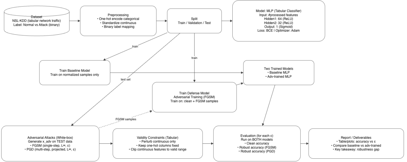
Figure 1: End-to-end adversarial ML pipeline for intrusion detection. Solid arrows indicate the primary data flow; dashed arrows indicate adversarial sample generation during training and evaluation.
