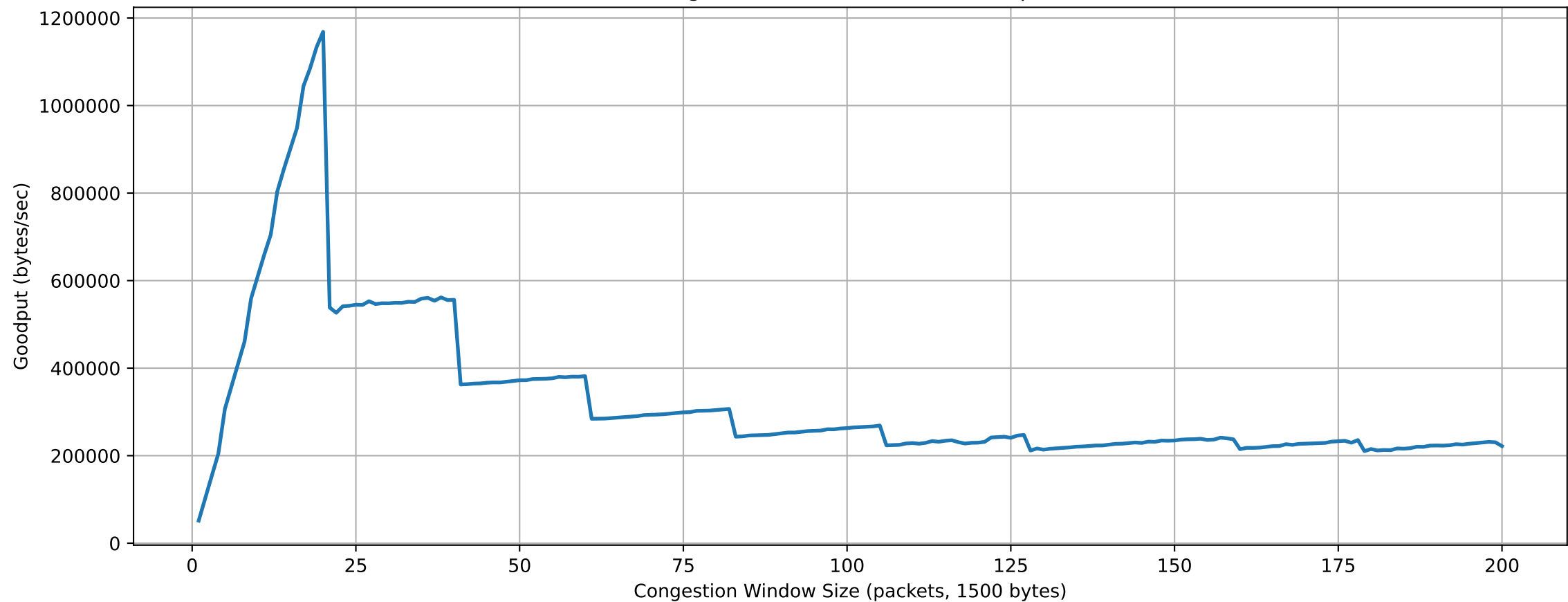
Congestion Window Size vs. Goodput
