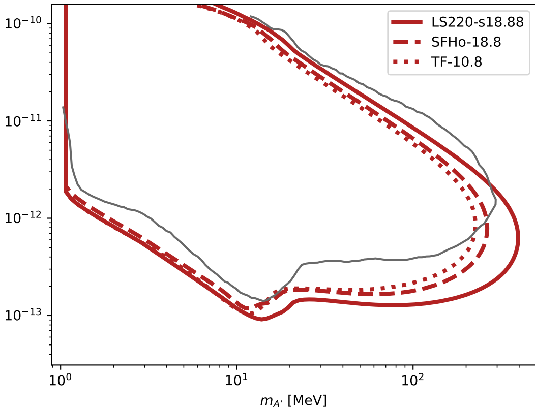
SN 2023ixf & v_w = 30 \text{ km s}^{-1}
