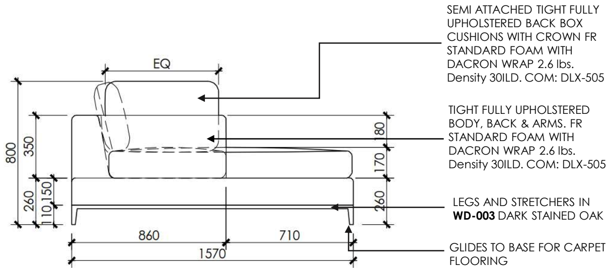
SIDE VIEW SCALE 1:20
