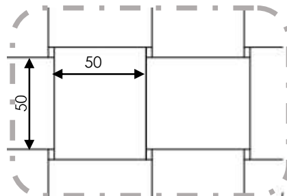
WEAVE LEATHER STRAP DETAILS
