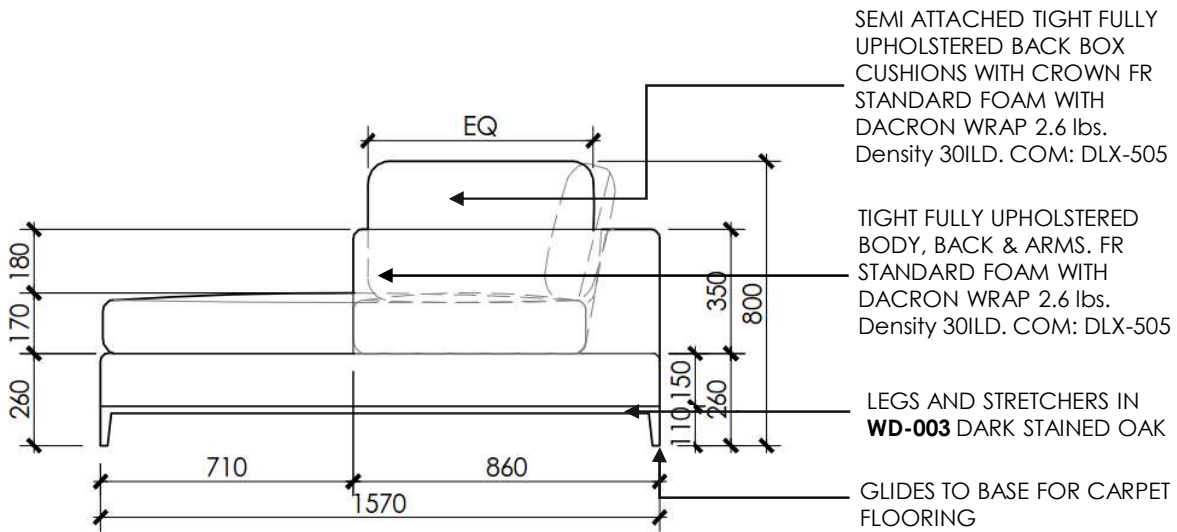
SIDE VIEW SCALE 1:20
