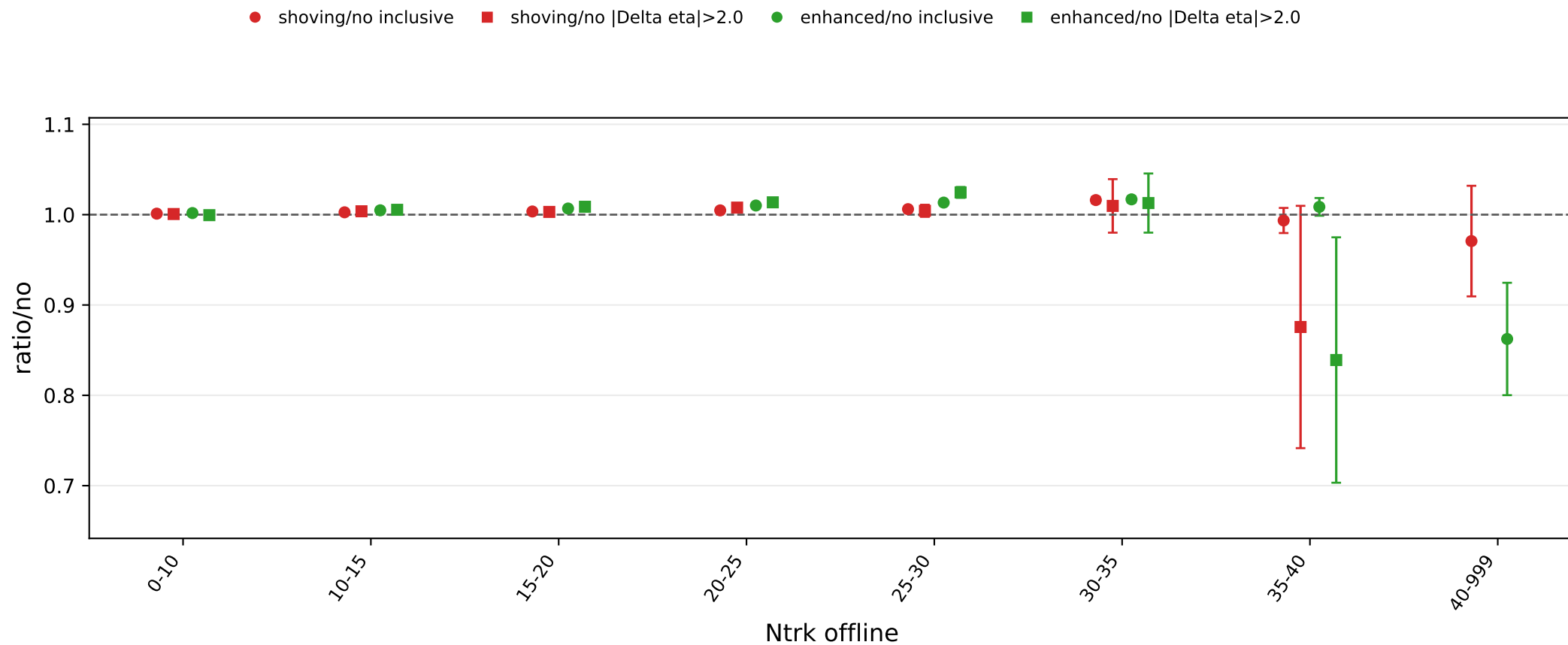
Pythia Z-pole 5M eta-gap comparison, |\Delta\eta| > 2.0 , beam axis sample ratios
