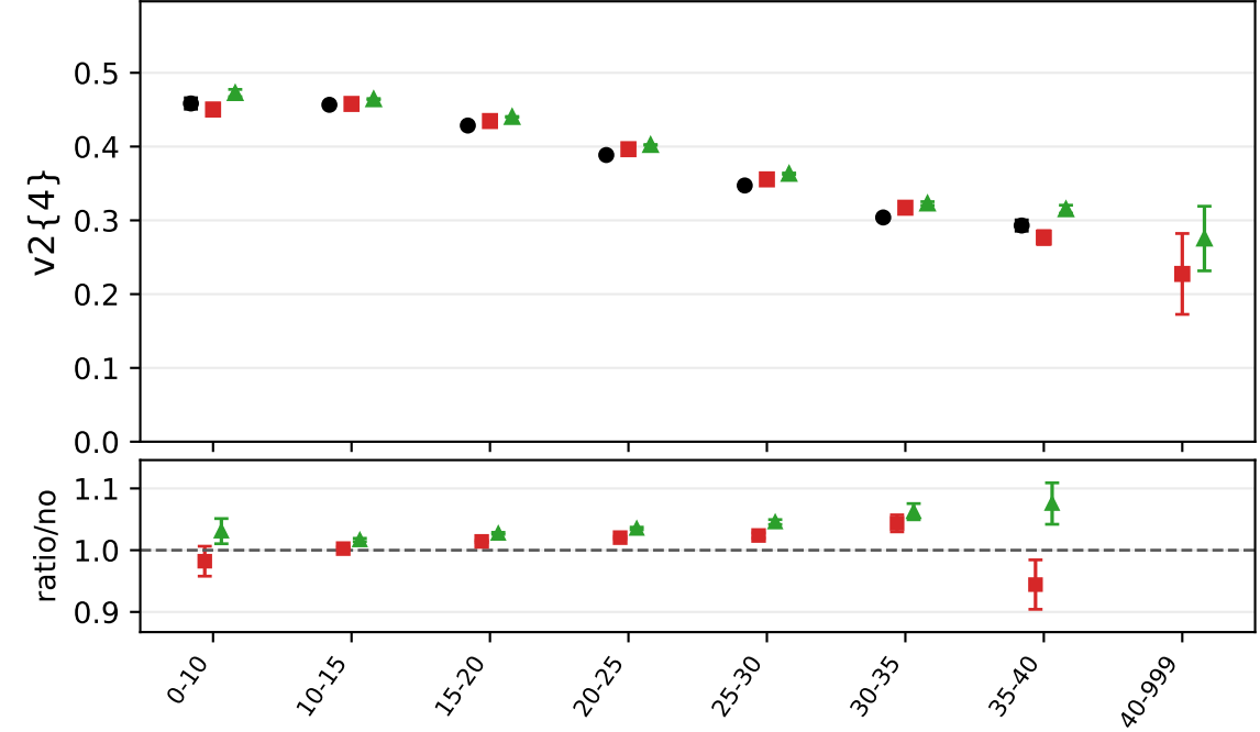
thrust axis, v2{4}
