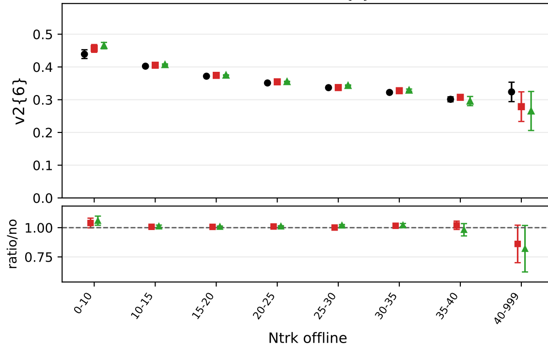
beam axis, v2{6}
