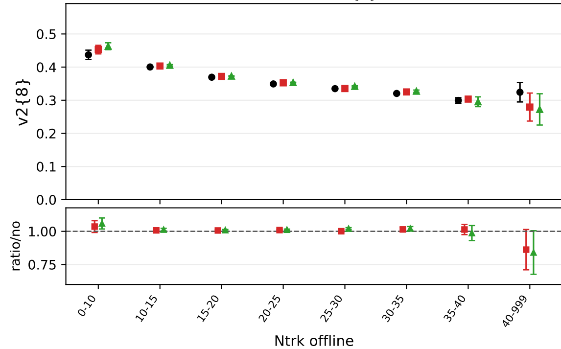
beam axis, v2{8}
