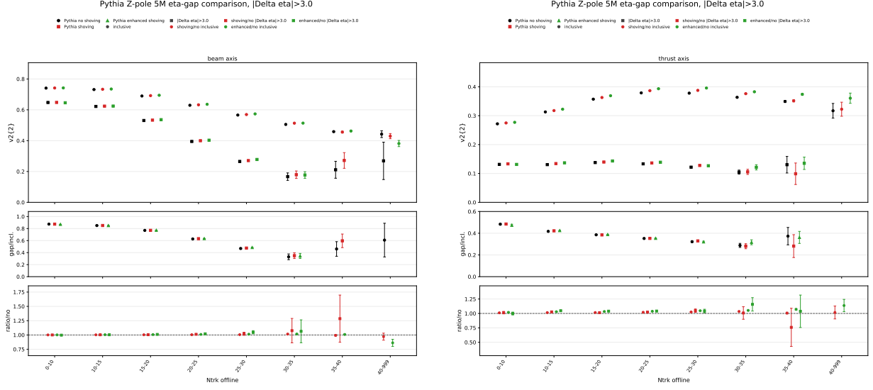
Figure 19: Generator-level Pythia no-shoving/nominal-shoving/factor-two-shoving comparison for Two-particle rapidity-gap selection |\Delta\eta| > 3.0 . Left: beam axis. Right: thrust axis.
