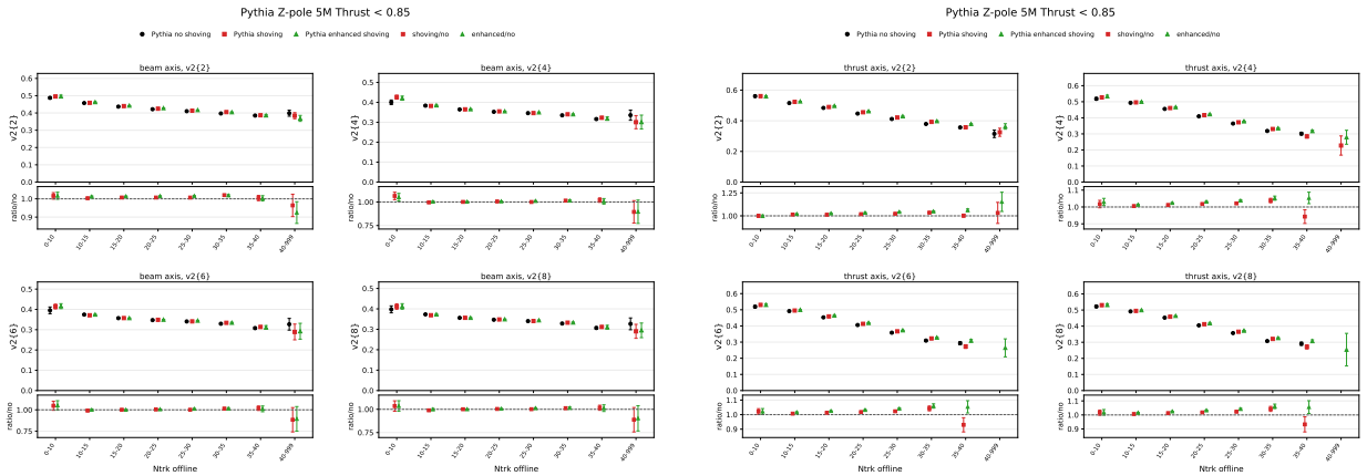
Figure 30: Generator-level Pythia no-shoving/nominal-shoving/factor-two-shoving comparison for Event-shape selection T < 0.85 . Left: beam axis. Right: thrust axis.
