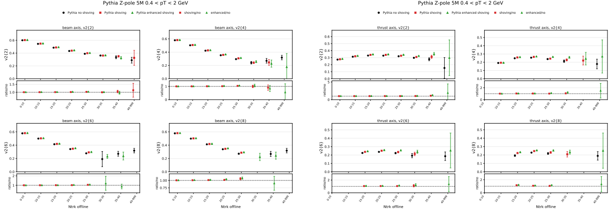
Figure 25: Generator-level Pythia no-shoving/nominal-shoving/factor-two-shoving comparison for Track selection 0.4 < p_T < 2 GeV. Left: beam axis. Right: thrust axis.
