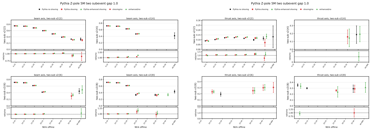
Figure 21: Generator-level Pythia no-shoving/nominal-shoving/factor-two-shoving comparison for Two-subevent cumulants with total excluded middle-region gap 1.0. Left: beam axis. Right: thrust axis.
