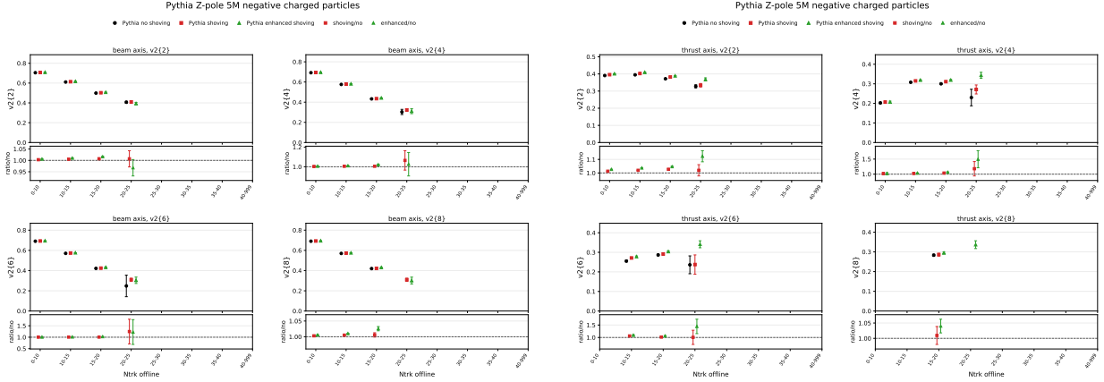
Figure 28: Generator-level Pythia no-shoving/nominal-shoving/factor-two-shoving comparison for Negative charged particles only. Left: beam axis. Right: thrust axis.
