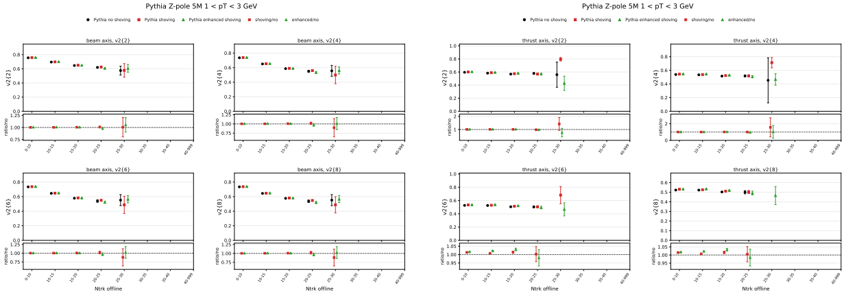
Figure 26: Generator-level Pythia no-shoving/nominal-shoving/factor-two-shoving comparison for Track selection 1 < p_T < 3 GeV. Left: beam axis. Right: thrust axis.
