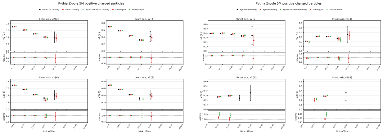
Figure 27: Generator-level Pythia no-shoving/nominal-shoving/factor-two-shoving comparison for Positive charged particles only. Left: beam axis. Right: thrust axis.
