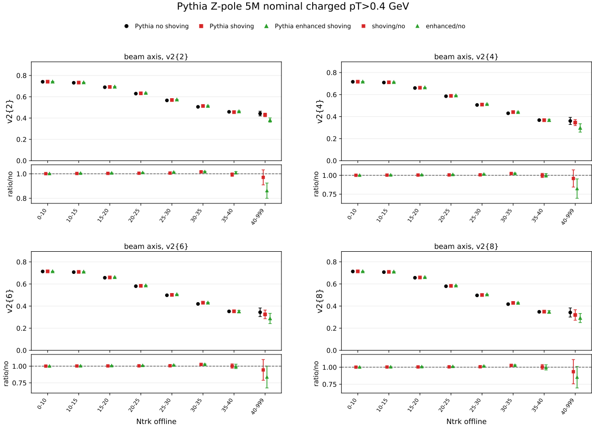
Figure 13: Generator-level Pythia comparison of beam-axis v_2\{m\} for no shoving, nominal Gleipnir shoving, and the factor-two shoving variation. All samples contain five million accepted hadronic Z-pole events and are processed with the same charged-particle selection and jackknife chunking. The lower panel in each observable pad gives the nominal/no-shoving and factor-two/no-shoving ratios.
