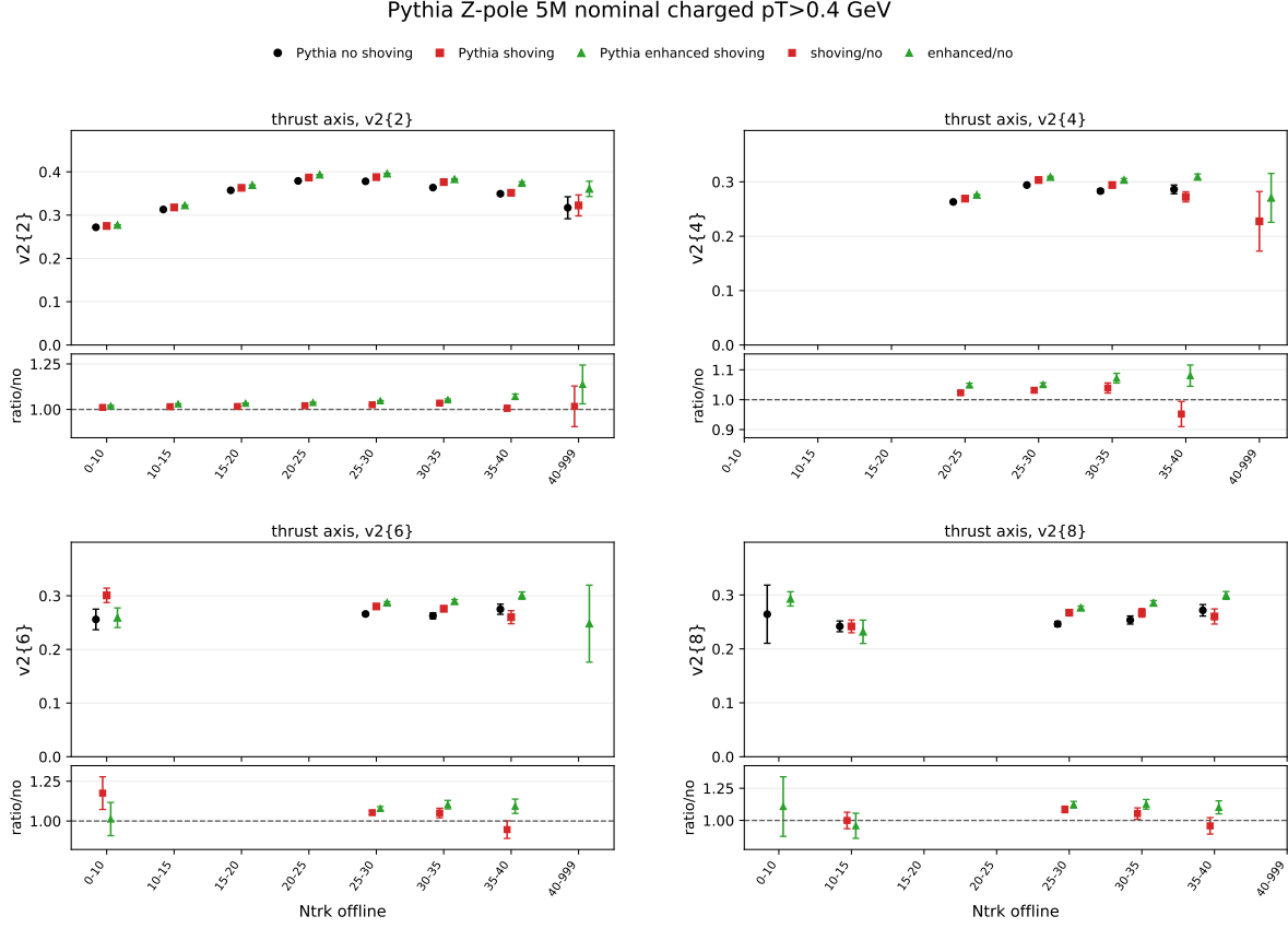
Figure 14: Generator-level Pythia comparison of thrust-axis v_2\{m\} for no shoving, nominal Gleipnir shoving, and the factor-two shoving variation. The shoving samples give a visible increase in the thrust-axis cumulants, especially for v_2\{2\} at intermediate multiplicity. The lower panel in each observable pad gives the nominal/no-shoving and factor-two/no-shoving ratios.
