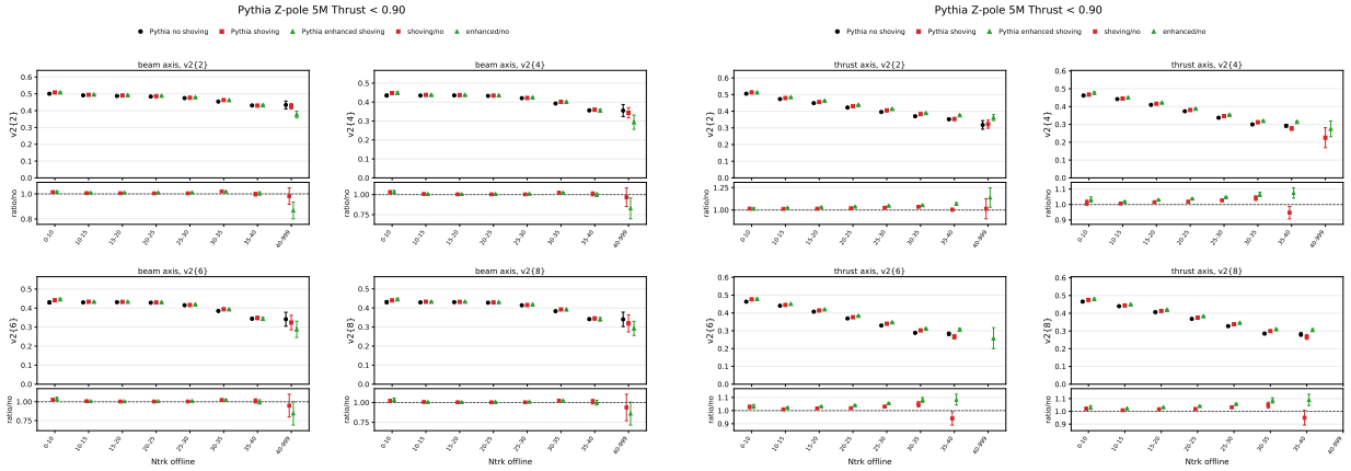
Figure 29: Generator-level Pythia no-shoving/nominal-shoving/factor-two-shoving comparison for Event-shape selection T < 0.90 . Left: beam axis. Right: thrust axis.
