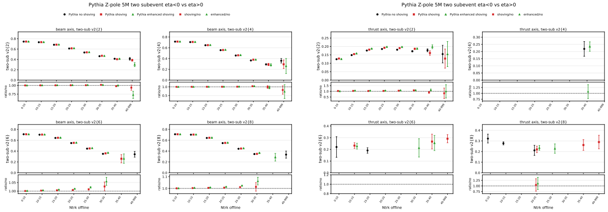
Figure 20: Generator-level Pythia no-shoving/nominal-shoving/factor-two-shoving comparison for Two-subevent cumulants with \eta < 0 versus \eta > 0 . Left: beam axis. Right: thrust axis.
