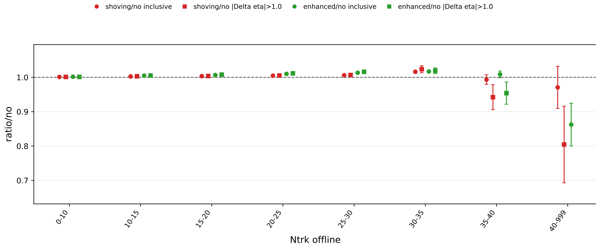
Pythia Z-pole 5M eta-gap comparison, |\Delta\eta|>1.0 , beam axis sample ratios
