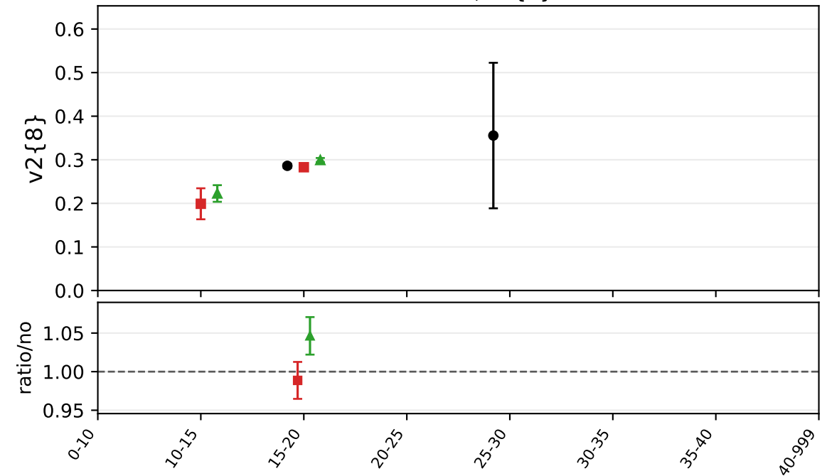
thrust axis, v2\{8\}
