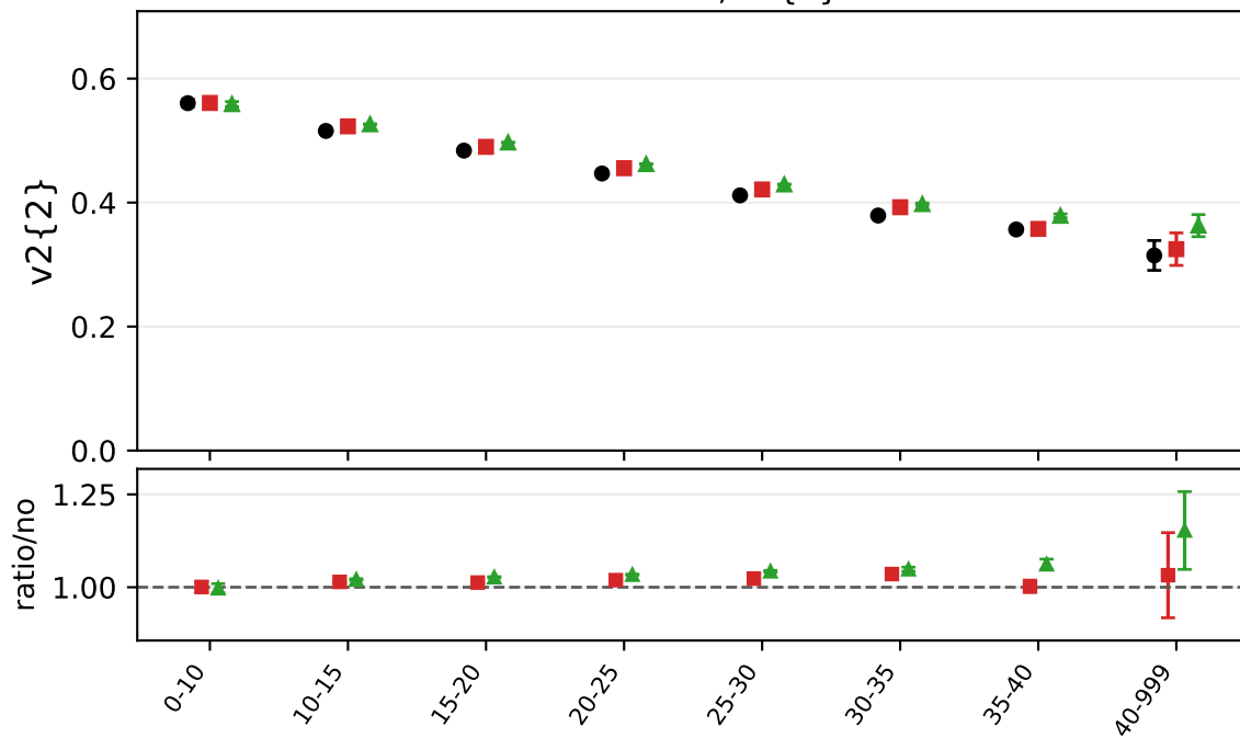
thrust axis, v2\{2\}
