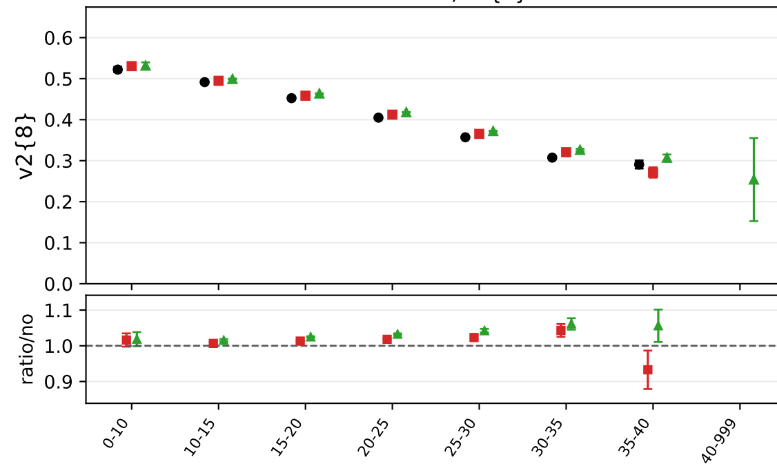
thrust axis, v2\{8\}
