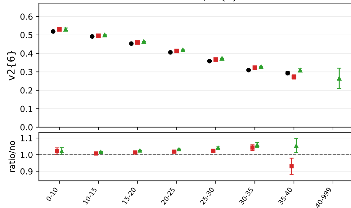
thrust axis, v2\{6\}
