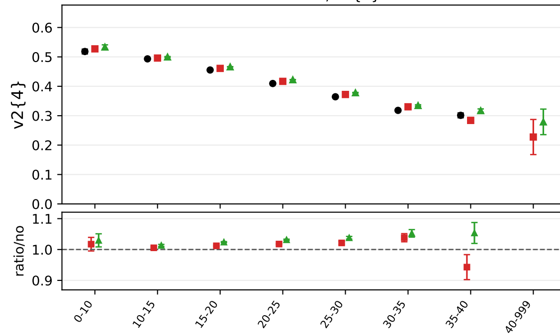
thrust axis, v2\{4\}
