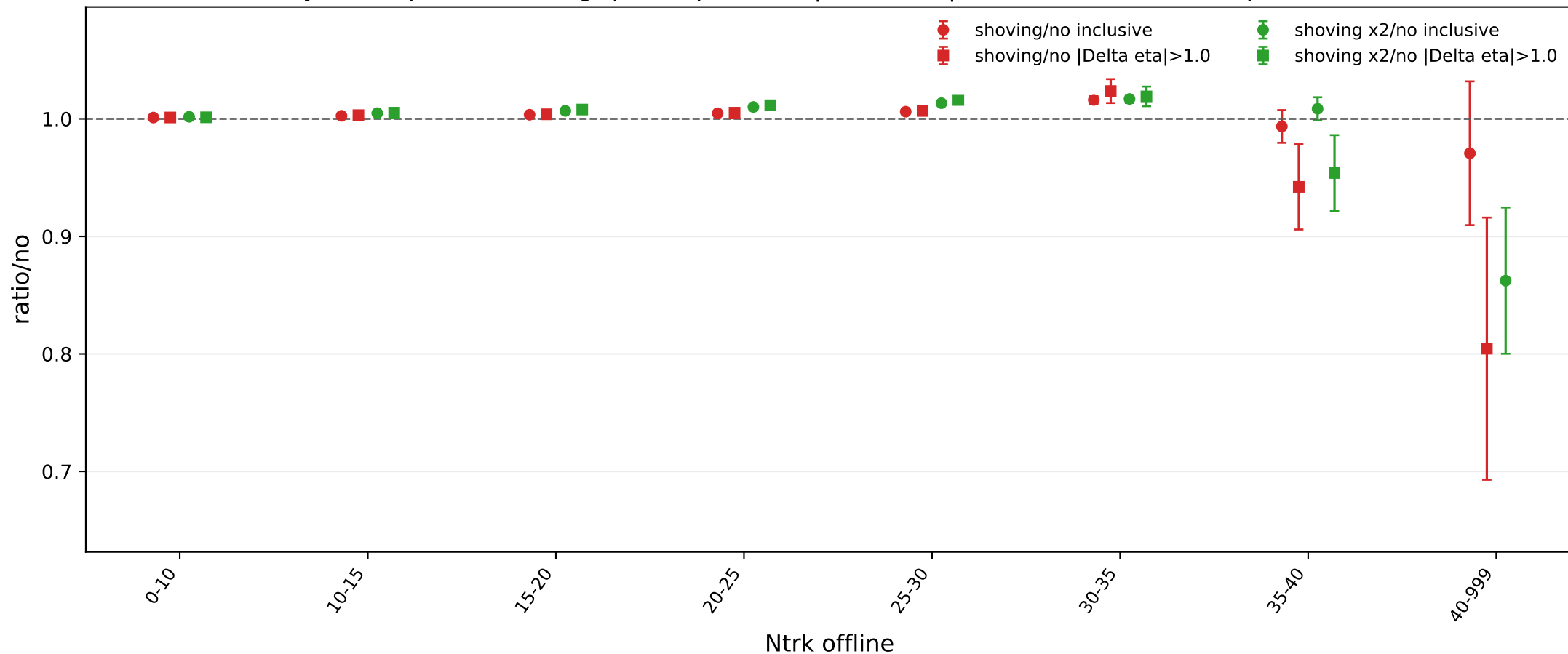
Pythia Z-pole 5M eta-gap comparison, |\Delta\eta| > 1.0 , beam axis sample ratios
