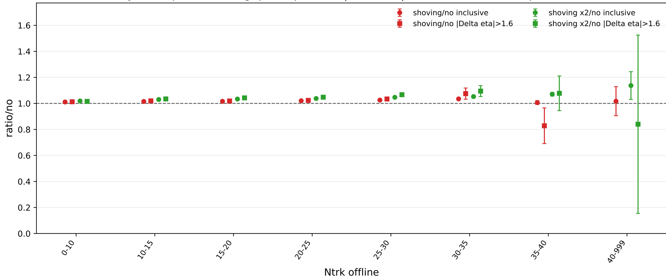
Pythia Z-pole 5M eta-gap comparison, |\Delta\eta| > 1.6 , thrust axis sample ratios
