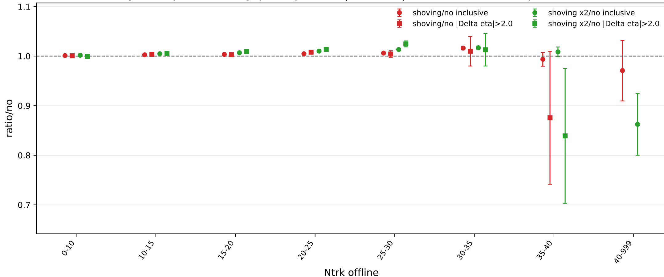
Pythia Z-pole 5M eta-gap comparison, |\Delta\eta| > 2.0 , beam axis sample ratios
