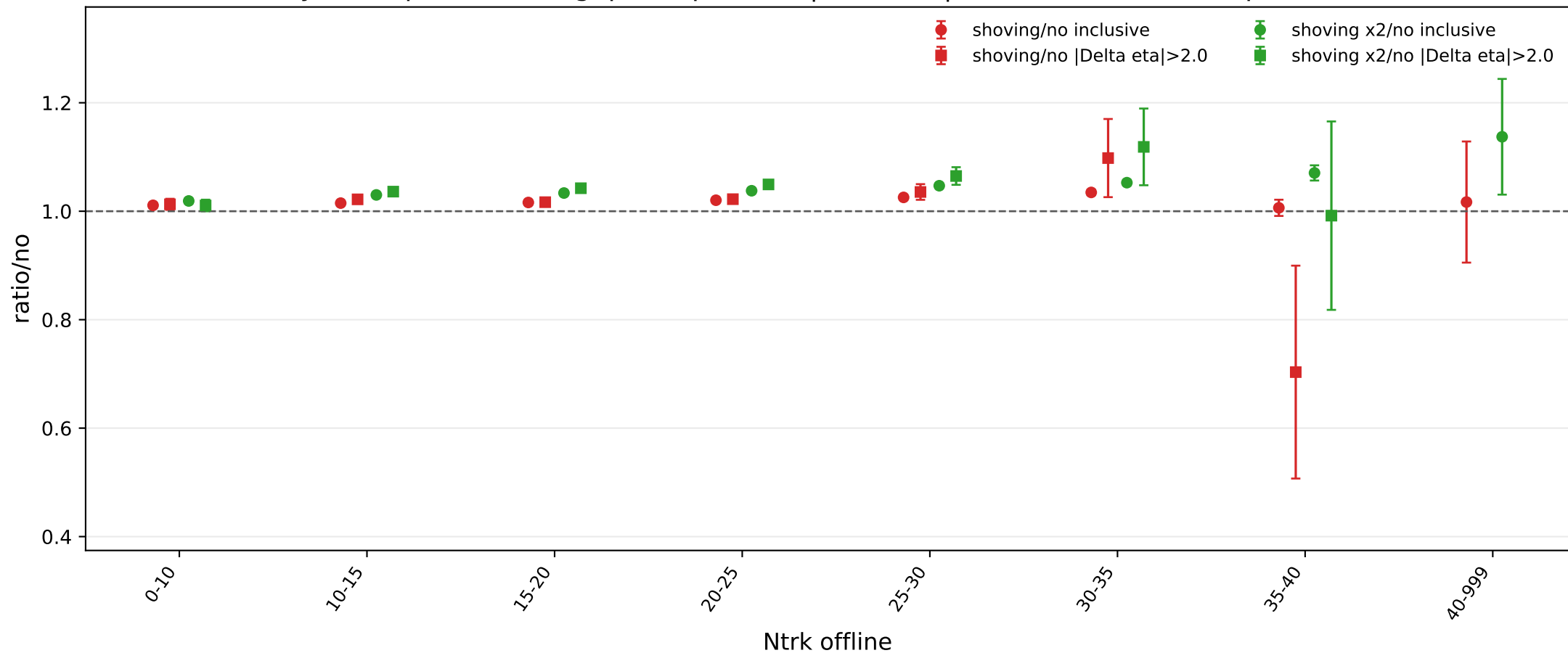
Pythia Z-pole 5M eta-gap comparison, |\Delta\eta| > 2.0 , thrust axis sample ratios
