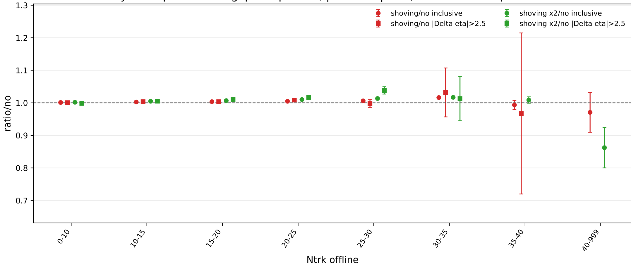
Pythia Z-pole 5M eta-gap comparison, |\Delta\eta| > 2.5 , beam axis sample ratios
