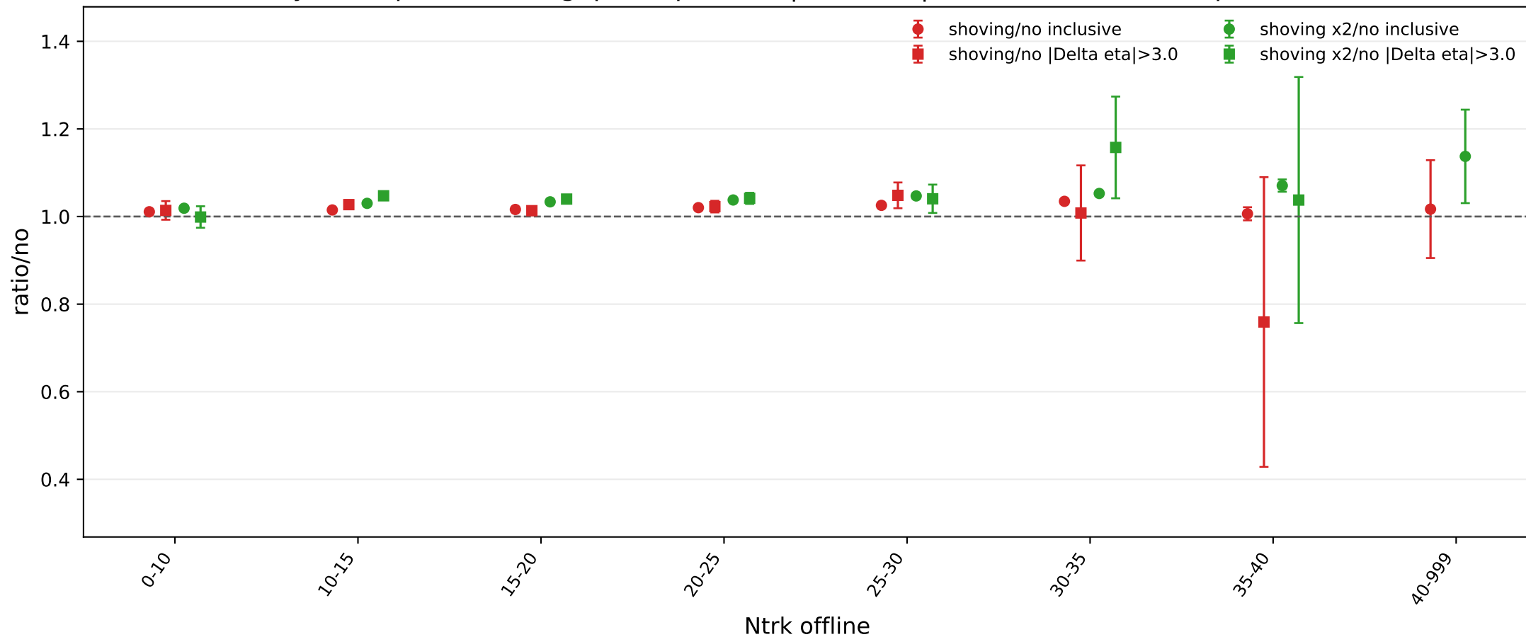
Pythia Z-pole 5M eta-gap comparison, |\Delta\eta| > 3.0 , thrust axis sample ratios
