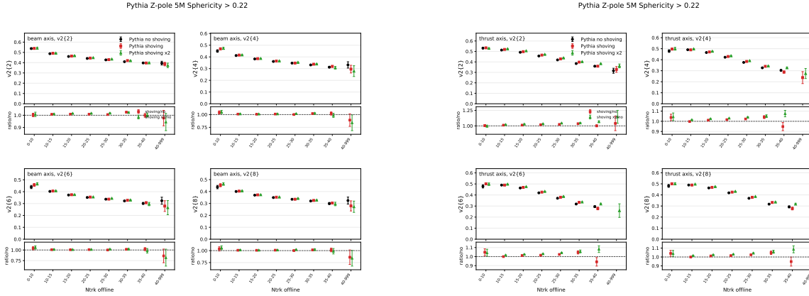
Figure 32: Generator-level Pythia no-shoving/nominal-shoving/factor-two-shoving comparison for Event-shape selection S > 0.22 . Left: beam axis. Right: thrust axis.
