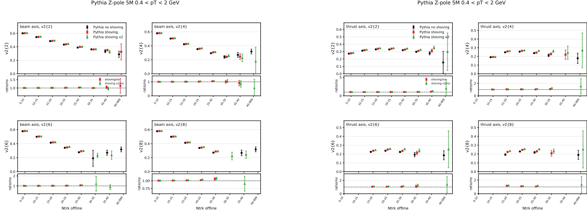
Figure 25: Generator-level Pythia no-shoving/nominal-shoving/factor-two-shoving comparison for Track selection 0.4 < p_T < 2 GeV. Left: beam axis. Right: thrust axis.
