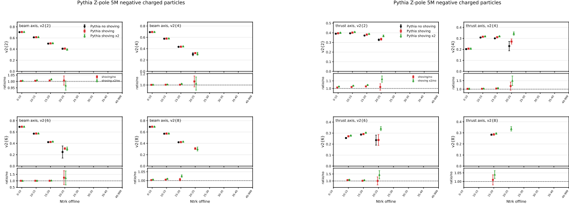
Figure 28: Generator-level Pythia no-shoving/nominal-shoving/factor-two-shoving comparison for Negative charged particles only. Left: beam axis. Right: thrust axis.
