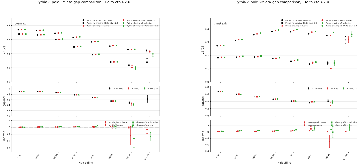
Figure 17: Generator-level Pythia no-shoving/nominal-shoving/factor-two-shoving comparison for Two-particle rapidity-gap selection |\Delta\eta| > 2.0 . Left: beam axis. Right: thrust axis.
