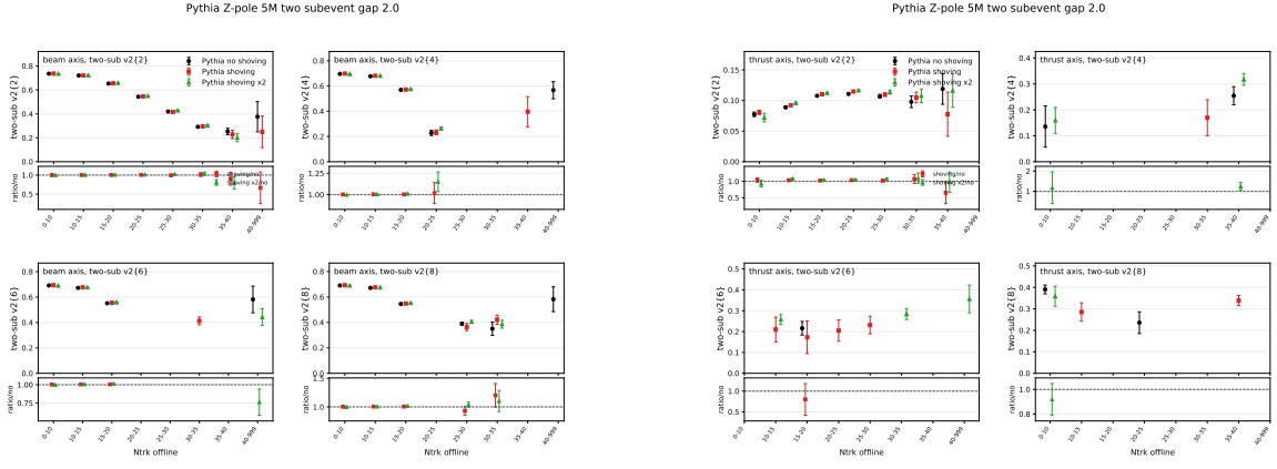
Figure 23: Generator-level Pythia no-shoving/nominal-shoving/factor-two-shoving comparison for Two-subevent cumulants with total excluded middle-region gap 2.0. Left: beam axis. Right: thrust axis.
