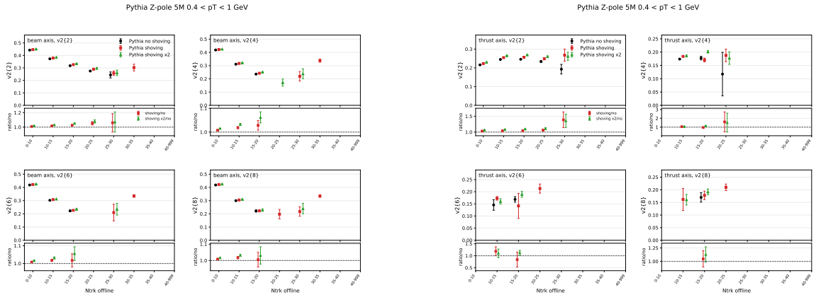
Figure 24: Generator-level Pythia no-shoving/nominal-shoving/factor-two-shoving comparison for Track selection 0.4 < p_T < 1 GeV. Left: beam axis. Right: thrust axis.
