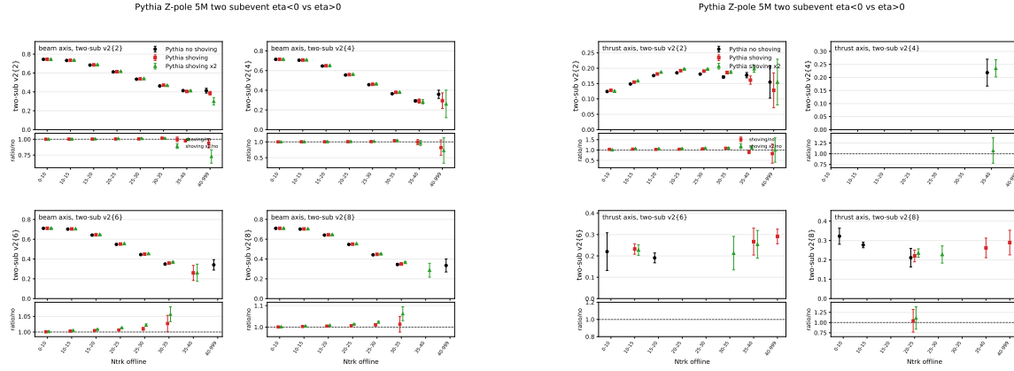
Figure 20: Generator-level Pythia no-shoving/nominal-shoving/factor-two-shoving comparison for Two-subevent cumulants with \eta < 0 versus \eta > 0 . Left: beam axis. Right: thrust axis.
