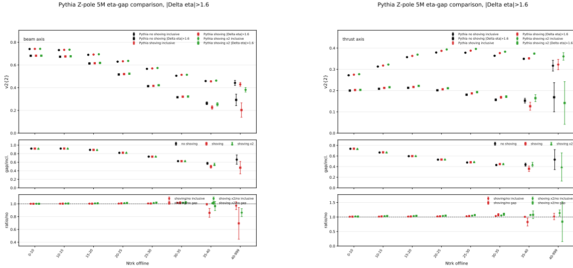
Figure 16: Generator-level Pythia no-shoving/nominal-shoving/factor-two-shoving comparison for Two-particle rapidity-gap selection |\Delta\eta| > 1.6 . Left: beam axis. Right: thrust axis.
