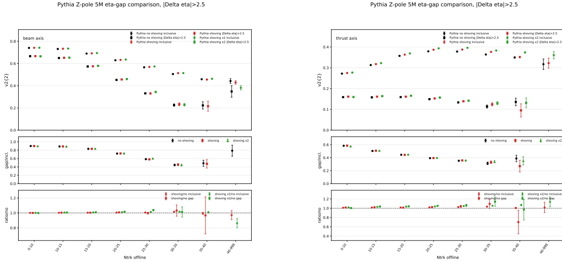
Figure 18: Generator-level Pythia no-shoving/nominal-shoving/factor-two-shoving comparison for Two-particle rapidity-gap selection |\Delta\eta| > 2.5 . Left: beam axis. Right: thrust axis.
