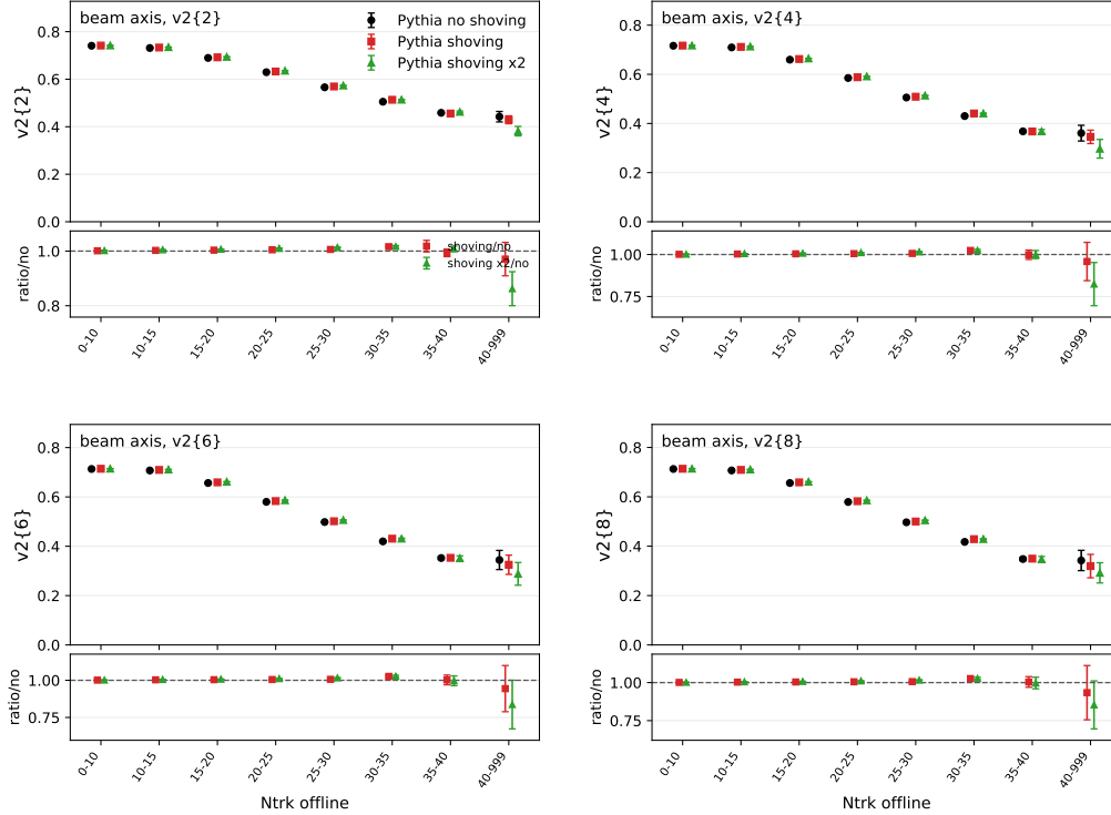
Figure 13: Generator-level Pythia comparison of beam-axis v_2\{m\} for no shoving, nominal Gleipnir shoving, and the factor-two shoving variation. All samples contain five million accepted hadronic Z-pole events and are processed with the same charged-particle selection and jackknife chunking. The lower panel in each observable pad gives the nominal/no-shoving and factor-two/no-shoving ratios.
