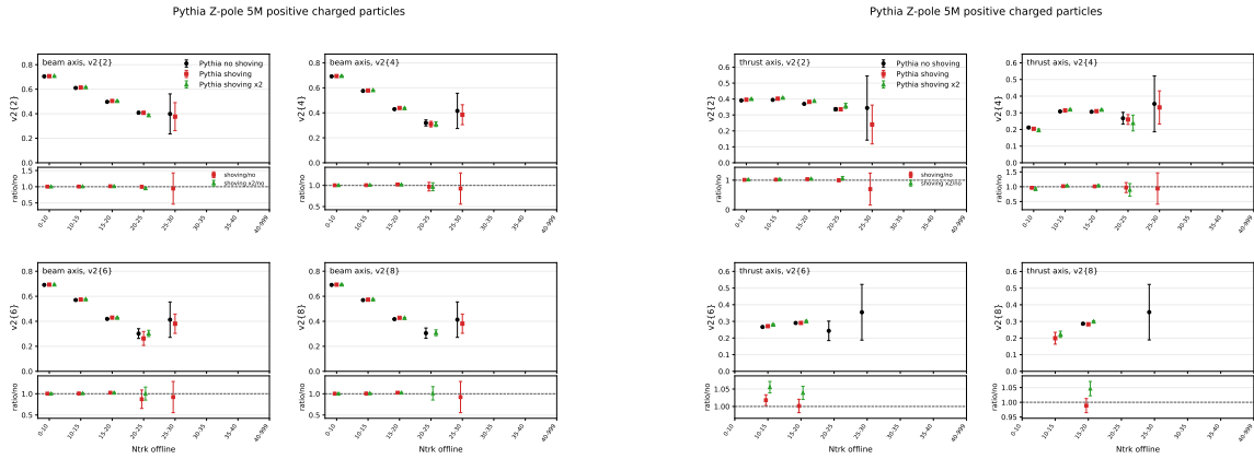
Figure 27: Generator-level Pythia no-shoving/nominal-shoving/factor-two-shoving comparison for Positive charged particles only. Left: beam axis. Right: thrust axis.
