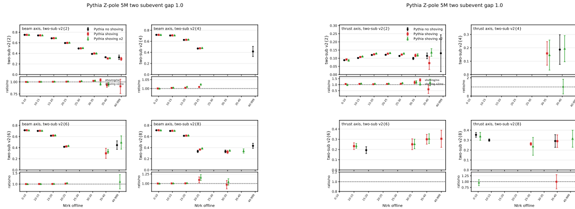
Figure 21: Generator-level Pythia no-shoving/nominal-shoving/factor-two-shoving comparison for Two-subevent cumulants with total excluded middle-region gap 1.0. Left: beam axis. Right: thrust axis.
