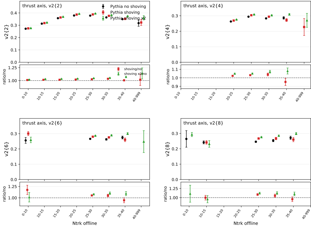
Figure 14: Generator-level Pythia comparison of thrust-axis v_2\{m\} for no shoving, nominal Gleipnir shoving, and the factor-two shoving variation. The shoving samples give a visible increase in the thrust-axis cumulants, especially for v_2\{2\} at intermediate multiplicity. The lower panel in each observable pad gives the nominal/no-shoving and factor-two/no-shoving ratios.
