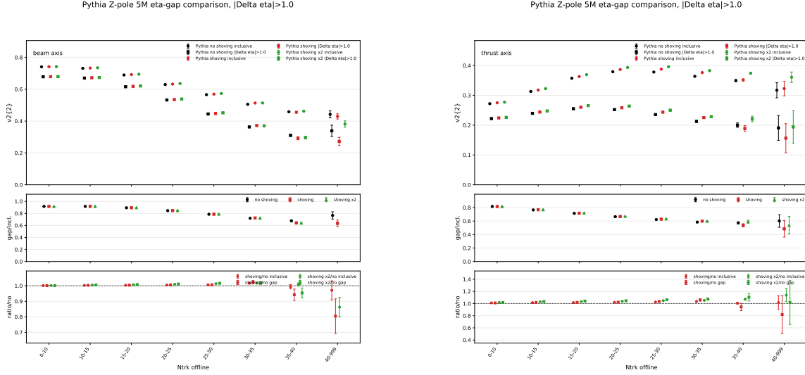
Figure 15: Generator-level Pythia no-shoving/nominal-shoving/factor-two-shoving comparison for Two-particle rapidity-gap selection |\Delta\eta| > 1.0 . Left: beam axis. Right: thrust axis.
