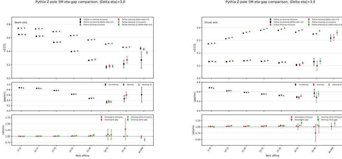
Figure 19: Generator-level Pythia no-shoving/nominal-shoving/factor-two-shoving comparison for Two-particle rapidity-gap selection |\Delta\eta| > 3.0 . Left: beam axis. Right: thrust axis.
