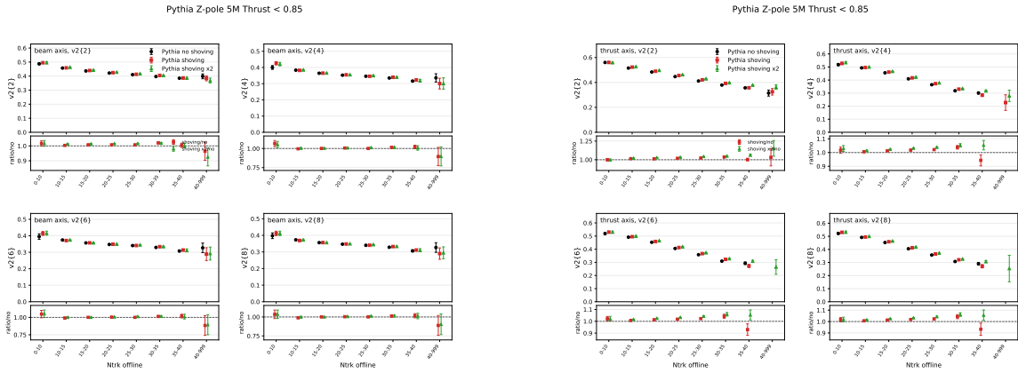
Figure 30: Generator-level Pythia no-shoving/nominal-shoving/factor-two-shoving comparison for Event-shape selection T < 0.85 . Left: beam axis. Right: thrust axis.
