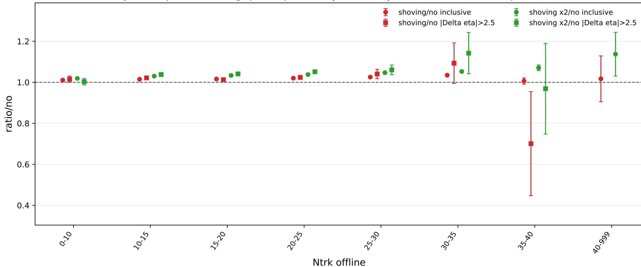
Pythia Z-pole 5M eta-gap comparison, |\Delta\eta| > 2.5 , thrust axis sample ratios
