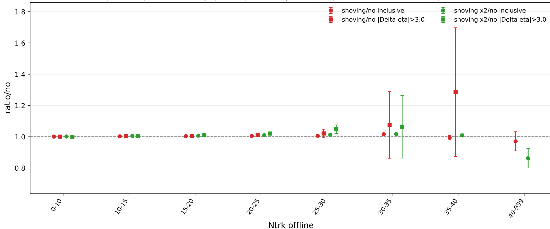
Pythia Z-pole 5M eta-gap comparison, |\Delta\eta| > 3.0 , beam axis sample ratios
