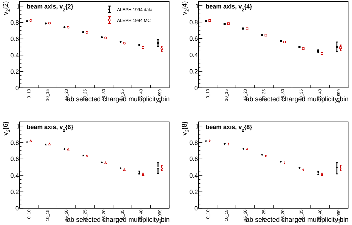
Figure 5: Beam-axis comparison of matched LEP1 1994 data and reconstructed MC. Each panel shows one cumulant order, with data and MC offset slightly in the lab-selected charged-multiplicity bin for readability.
