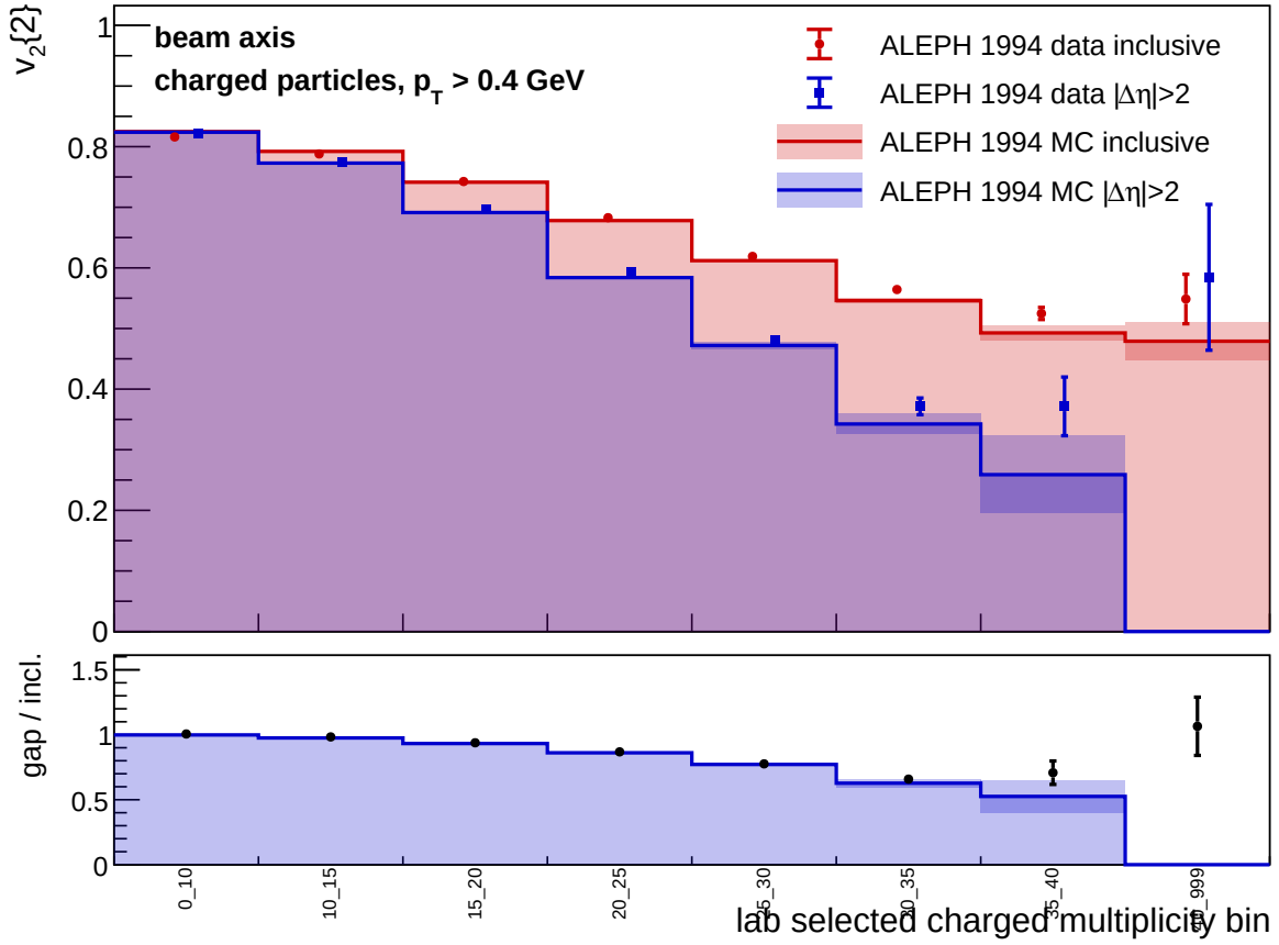
Figure 7: Beam-axis comparison of inclusive v_2\{2\} and v_2\{2, |\Delta\eta| > 2\} for matched LEP1 1994 data and reconstructed MC. MC is shown as histogram bands and data as points. The lower panel shows the rapidity-gap value divided by the inclusive value.
