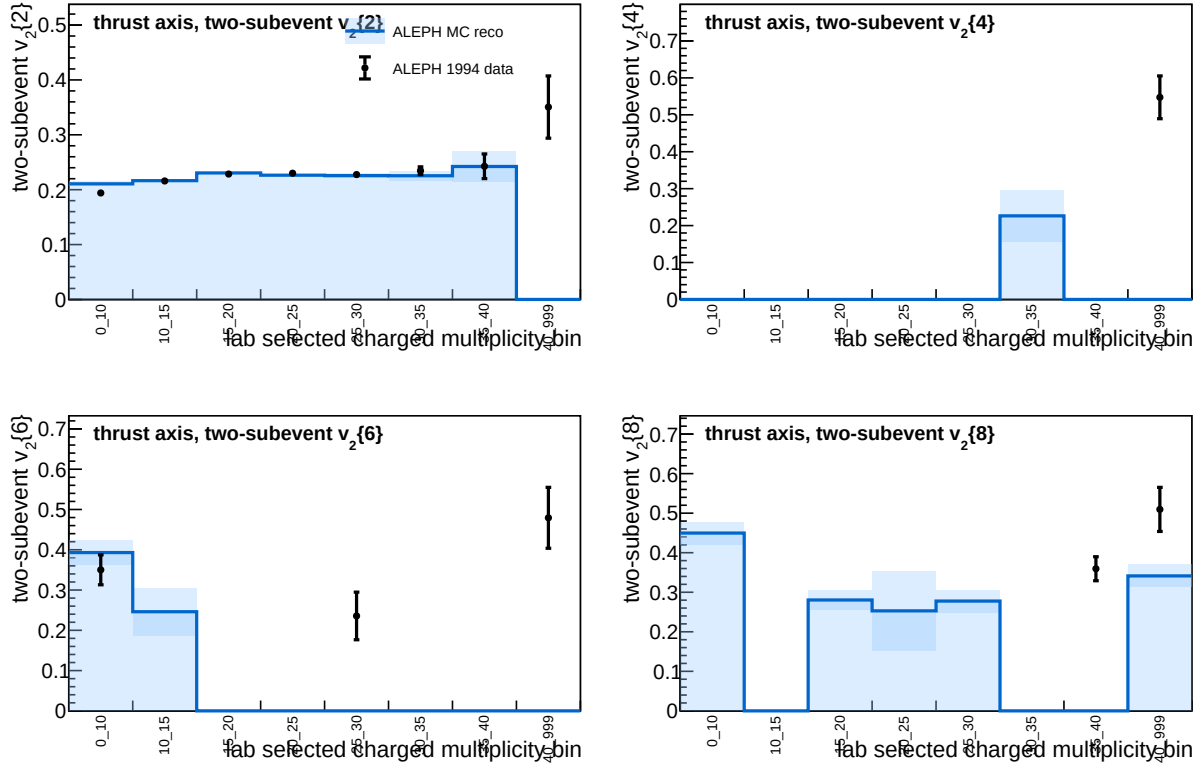
Figure 10: Thrust-axis two-subevent comparison of matched LEP1 1994 data and reconstructed MC. Missing or zero high-order entries correspond to sign-invalid cumulants or bins without a valid real-valued v_2\{2k\}_{2\text{sub}} .
