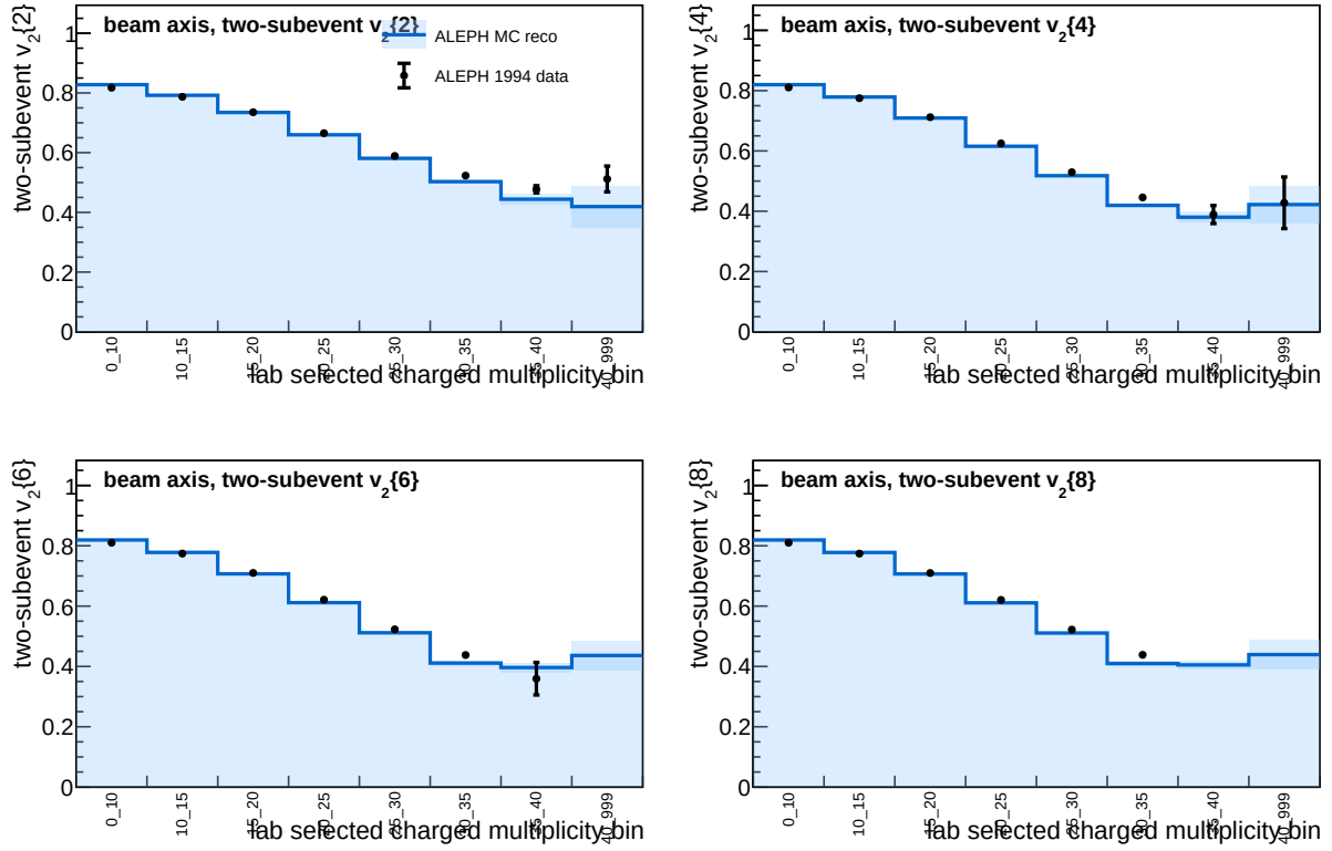
Figure 9: Beam-axis two-subevent comparison of matched LEP1 1994 data and reconstructed MC. MC is drawn as a histogram with statistical band, while data are shown as points with delete-one-chunk jackknife uncertainties.
