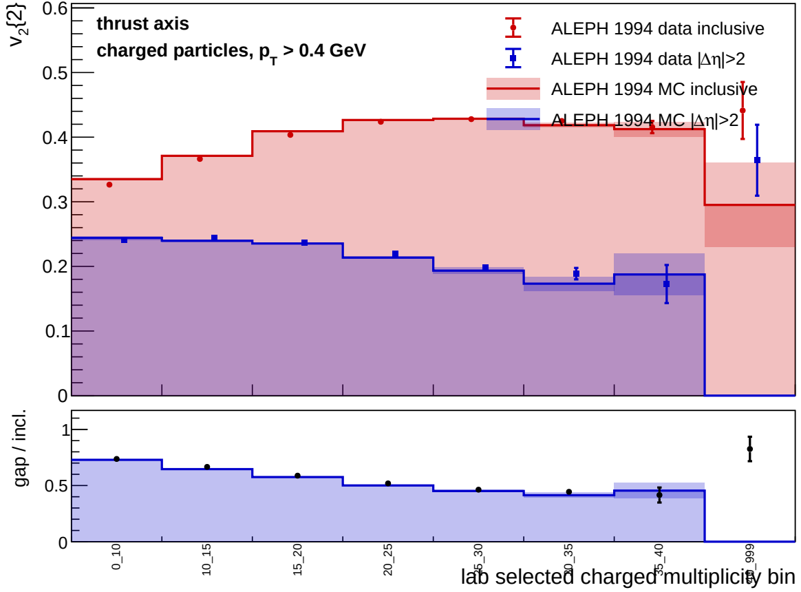
Figure 8: Thrust-axis comparison of inclusive v_2\{2\} and v_2\{2, |\Delta\eta| > 2\} for matched LEP1 1994 data and reconstructed MC. The rapidity gap is evaluated using pseudorapidity around the thrust axis; the multiplicity bin remains the selected laboratory charged-particle multiplicity.
