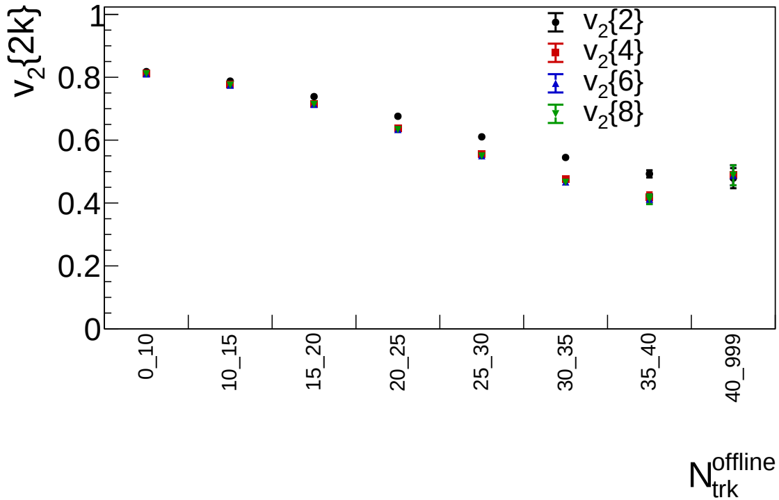
Figure 3: LEP1 1994 reconstructed-MC v_2\{2\} , v_2\{4\} , v_2\{6\} , and v_2\{8\} versus selected charged-particle multiplicity using the laboratory beam-axis azimuth.
