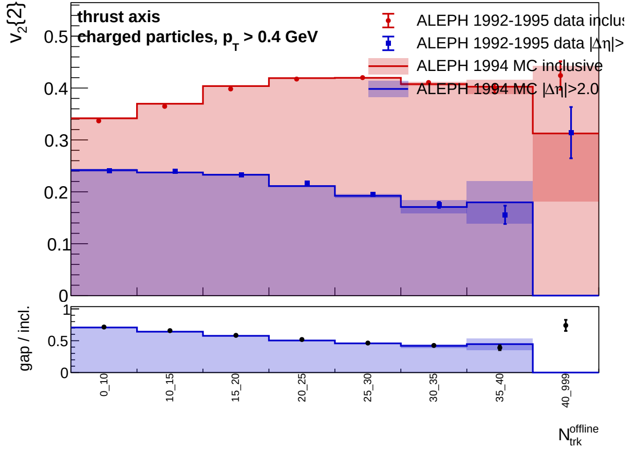
Figure 8: Thrust-axis comparison of inclusive v_2\{2\} and v_2\{2, |\Delta\eta| > 2\} for LEP1 1992–1995 data and 1994 reconstructed MC. The rapidity gap is evaluated using pseudorapidity around the thrust axis; the multiplicity bin remains the selected laboratory charged-particle multiplicity.
