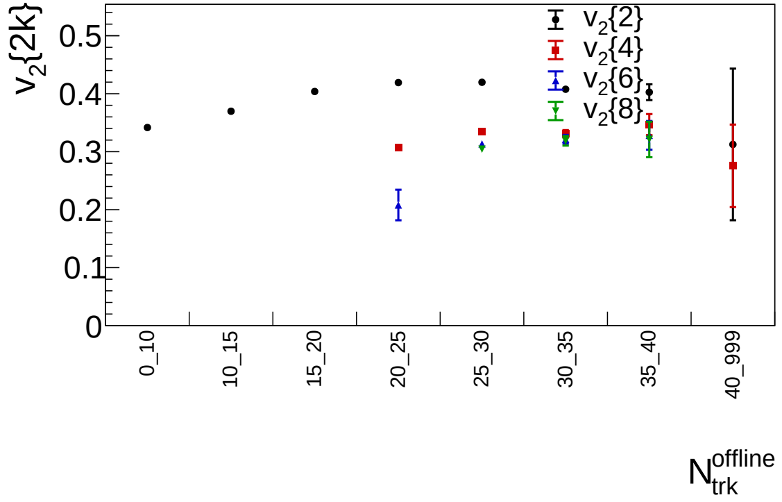
Figure 6: LEP1 1994 reconstructed-MC v_2\{2\} , v_2\{4\} , v_2\{6\} , and v_2\{8\} versus selected charged-particle multiplicity using azimuth around the event thrust axis.
