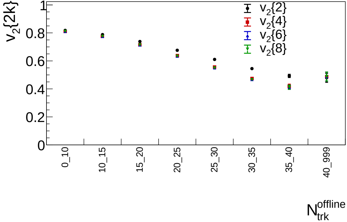
Figure 5: LEP1 1994 reconstructed-MC v_2\{2\} , v_2\{4\} , v_2\{6\} , and v_2\{8\} versus selected charged-particle multiplicity using the laboratory beam-axis azimuth.
