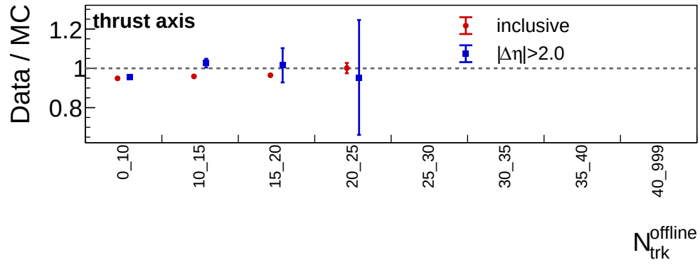
Figure 16: Thrust-axis v_2\{2\} comparison with 1 < p_T < 3 GeV selected charged particles. The rapidity-gap observable uses |\Delta\eta| > 2.0 in the thrust-axis coordinate frame.
