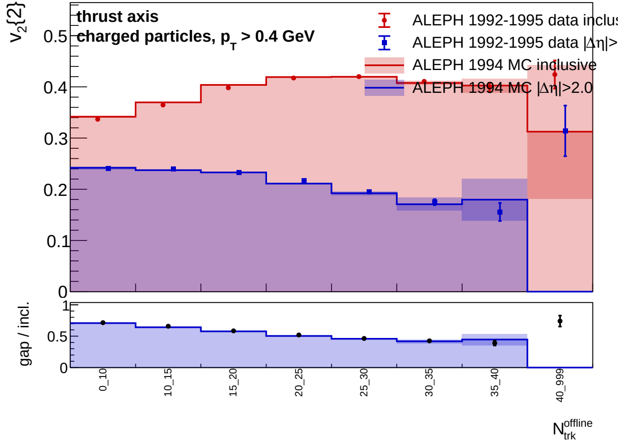
Figure 10: Thrust-axis comparison of inclusive v_2\{2\} and v_2\{2, |\Delta\eta| > 2\} for LEP1 1992–1995 data and 1994 reconstructed MC. The rapidity gap is evaluated using pseudorapidity around the thrust axis; the multiplicity bin remains the selected laboratory charged-particle multiplicity.
