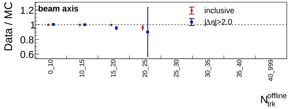
Figure 15: Beam-axis v_2\{2\} comparison with 1 < p_T < 3 GeV selected charged particles. The rapidity-gap observable uses |\Delta\eta| > 2.0 .
