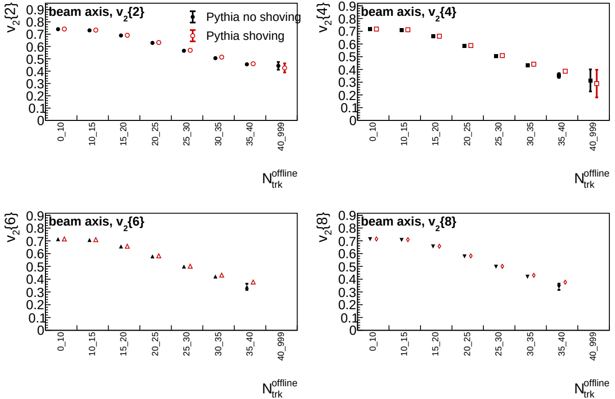
Figure 13: Generator-level Pythia comparison of beam-axis v_2\{m\} with and without Gleipnir shoving. Both samples contain one million accepted hadronic Z-pole events and are processed with the same charged-particle selection and jackknife chunking.
