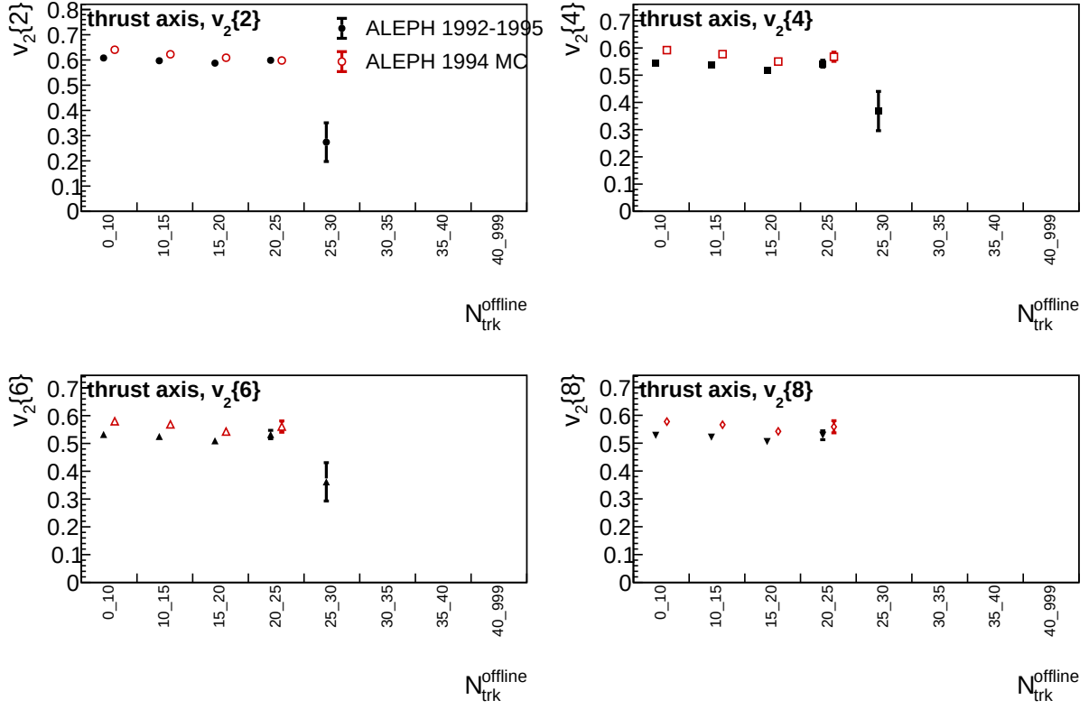
Figure 20: Thrust-axis comparison of v_2\{2\} , v_2\{4\} , v_2\{6\} , and v_2\{8\} for LEP1 1992–1995 data and 1994 reconstructed MC using selected charged particles with 1 < p_T < 3 GeV, where p_T is evaluated relative to the thrust axis.
