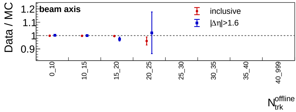
Figure 15: Beam-axis v_2\{2\} comparison with 1 < p_T < 3 GeV selected charged particles and |\Delta\eta| > 1.6 .
