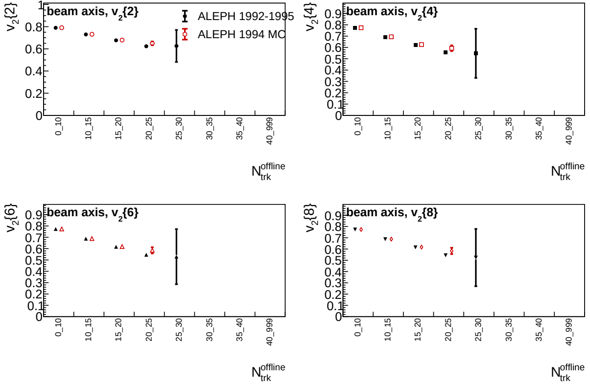
Figure 17: Beam-axis comparison of v_2\{2\} , v_2\{4\} , v_2\{6\} , and v_2\{8\} for LEP1 1992–1995 data and 1994 reconstructed MC using selected charged particles with 1 < p_T < 3 GeV.
