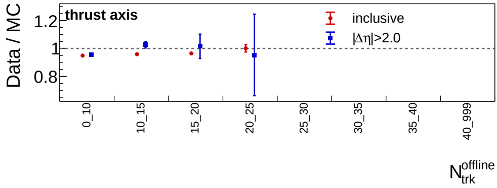
Figure 20: Thrust-axis v_2\{2\} comparison with 1 < p_T < 3 GeV selected charged particles. The rapidity-gap observable uses |\Delta\eta| > 2.0 in the thrust-axis coordinate frame.
