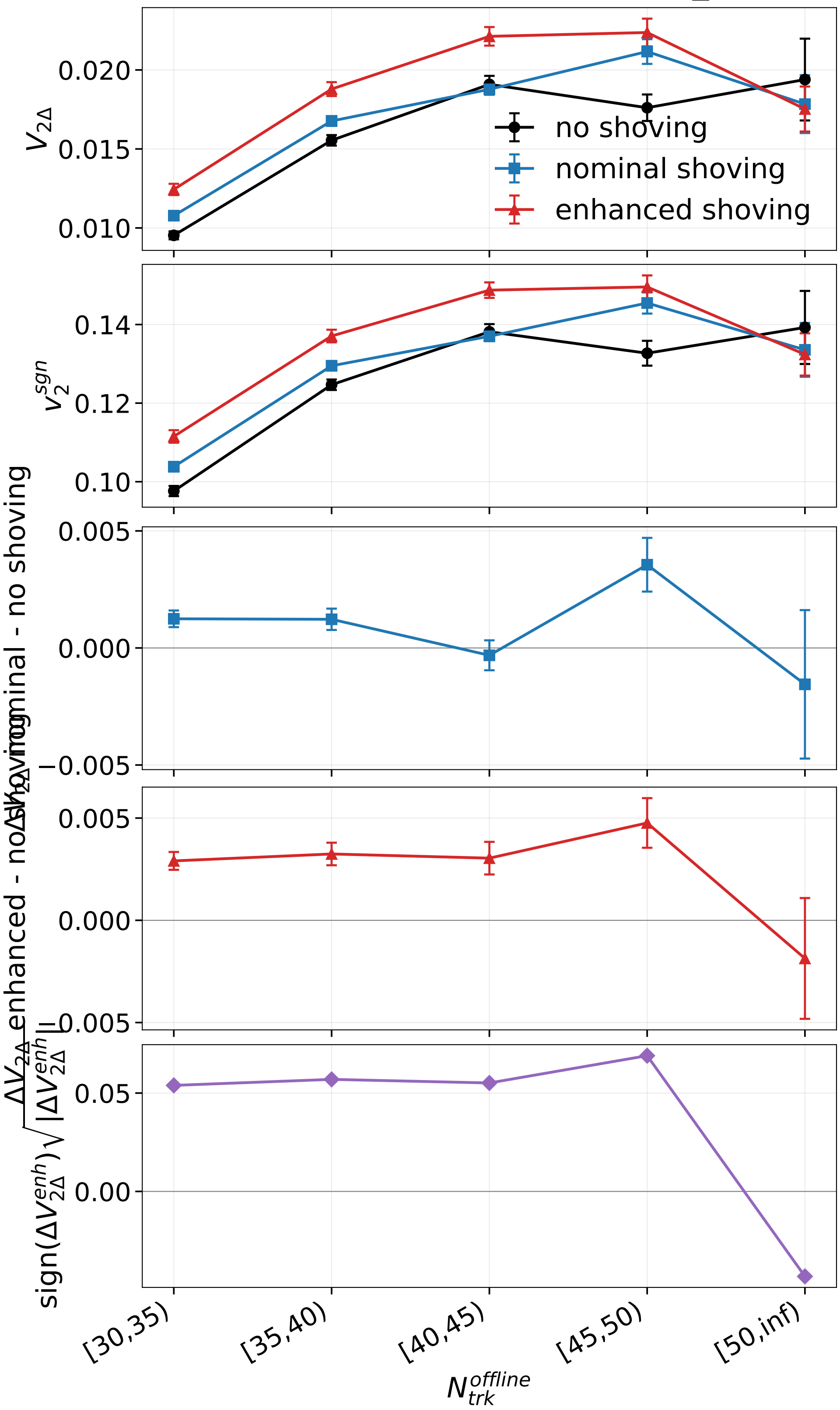
0 GeV long-range thrust-axis V2Delta, high_multiplicity
