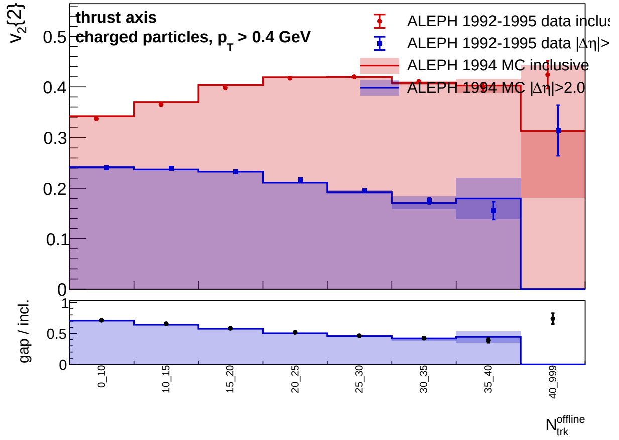
Figure 12: Thrust-axis comparison of inclusive v_2\{2\} and v_2\{2, |\Delta\eta| > 2\} for LEP1 1992–1995 data and 1994 reconstructed MC. The rapidity gap is evaluated using pseudorapidity around the thrust axis; the multiplicity bin remains the selected laboratory charged-particle multiplicity.
