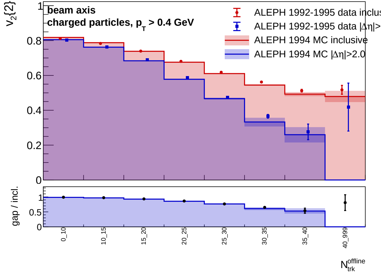
Figure 11: Beam-axis comparison of inclusive v_2\{2\} and v_2\{2, |\Delta\eta| > 2\} for LEP1 1992–1995 data and 1994 reconstructed MC. MC is shown as histogram bands and data as points. The lower panel shows the rapidity-gap value divided by the inclusive value.
