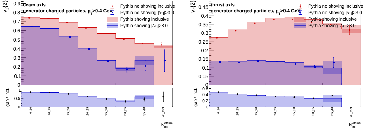
Figure 19: Generator-level Pythia no-shoving/shoving comparison for Two-particle rapidity-gap selection |\Delta\eta| > 3.0 . Left: beam axis. Right: thrust axis.
