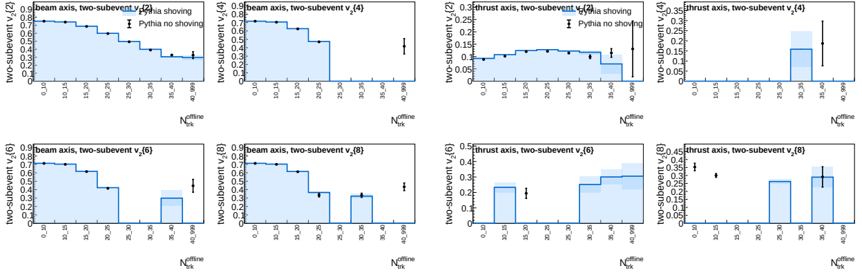
Figure 21: Generator-level Pythia no-shoving/shoving comparison for Two-subevent cumulants with total excluded middle-region gap 1.0. Left: beam axis. Right: thrust axis.
