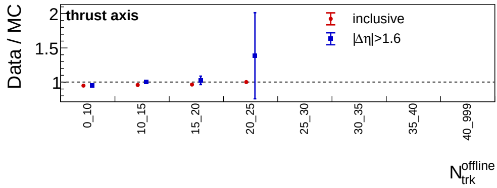
Figure 42: Thrust-axis v_2\{2\} comparison with 1 < p_T < 3 \text{ GeV} selected charged particles and |\Delta\eta| > 1.6 in the thrust-axis coordinate frame.
