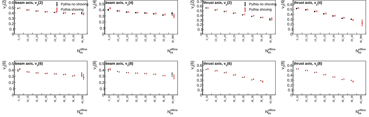
Figure 30: Generator-level Pythia no-shoving/shoving comparison for Event-shape selection T < 0.85 . Left: beam axis. Right: thrust axis.
