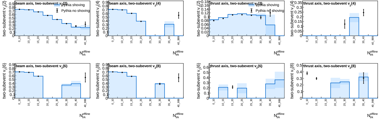
Figure 22: Generator-level Pythia no-shoving/shoving comparison for Two-subevent cumulants with total excluded middle-region gap 1.6. Left: beam axis. Right: thrust axis.
