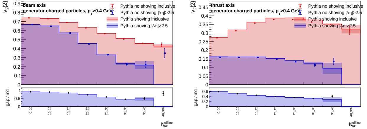
Figure 18: Generator-level Pythia no-shoving/shoving comparison for Two-particle rapidity-gap selection |\Delta\eta| > 2.5 . Left: beam axis. Right: thrust axis.
