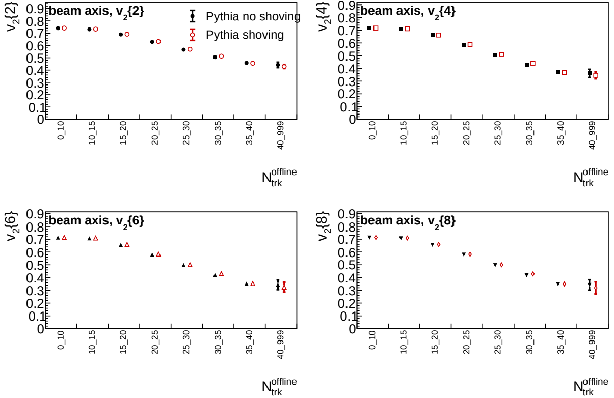
Figure 13: Generator-level Pythia comparison of beam-axis v_2\{m\} with and without Gleipnir shoving. Both samples contain five million accepted hadronic Z-pole events and are processed with the same charged-particle selection and jackknife chunking.
