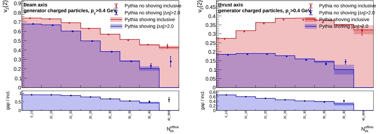
Figure 17: Generator-level Pythia no-shoving/shoving comparison for Two-particle rapidity-gap selection |\Delta\eta| > 2.0 . Left: beam axis. Right: thrust axis.
