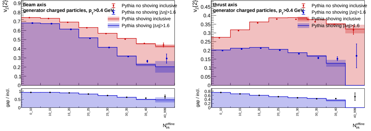
Figure 16: Generator-level Pythia no-shoving/shoving comparison for Two-particle rapidity-gap selection |\Delta\eta| > 1.6 . Left: beam axis. Right: thrust axis.
