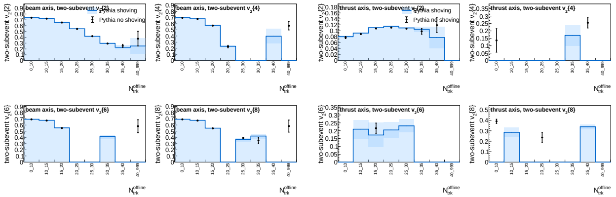
Figure 23: Generator-level Pythia no-shoving/shoving comparison for Two-subevent cumulants with total excluded middle-region gap 2.0. Left: beam axis. Right: thrust axis.
