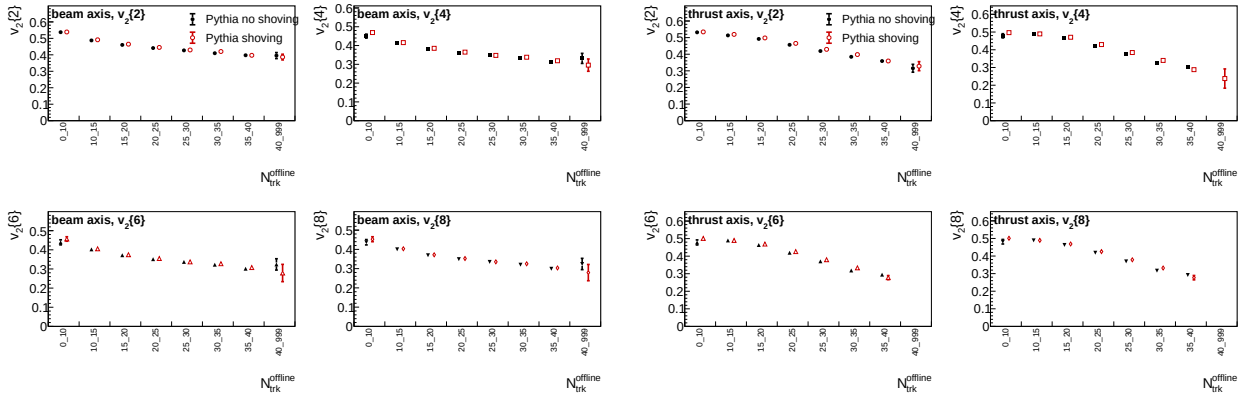
Figure 32: Generator-level Pythia no-shoving/shoving comparison for Event-shape selection S > 0.22 . Left: beam axis. Right: thrust axis.
