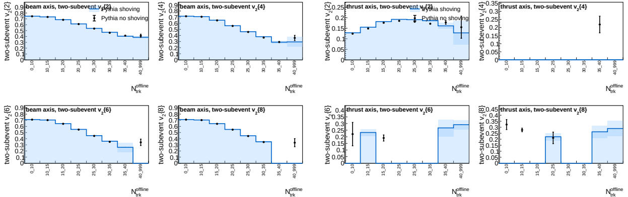
Figure 20: Generator-level Pythia no-shoving/shoving comparison for Two-subevent cumulants with \eta < 0 versus \eta > 0 . Left: beam axis. Right: thrust axis.
