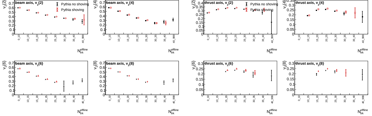
Figure 25: Generator-level Pythia no-shoving/shoving comparison for Track selection 0.4 < p_T < 2 GeV. Left: beam axis. Right: thrust axis.
