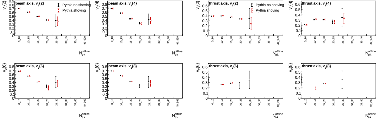
Figure 27: Generator-level Pythia no-shoving/shoving comparison for Positive charged particles only. Left: beam axis. Right: thrust axis.
