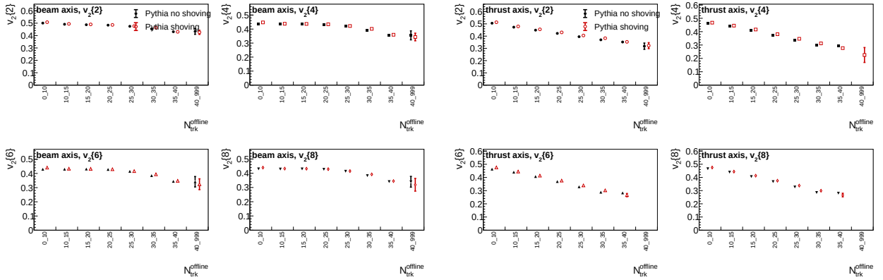
Figure 29: Generator-level Pythia no-shoving/shoving comparison for Event-shape selection T < 0.90 . Left: beam axis. Right: thrust axis.
