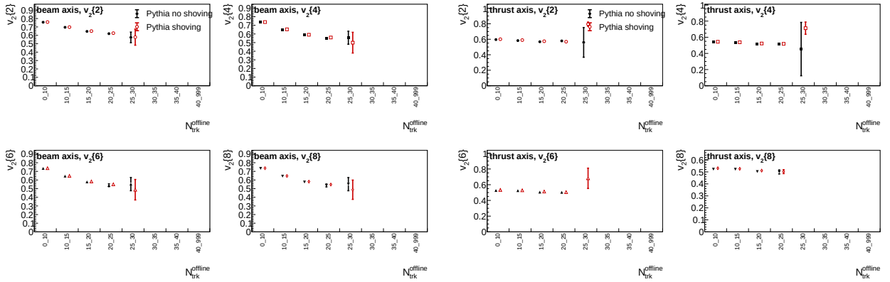
Figure 26: Generator-level Pythia no-shoving/shoving comparison for Track selection 1 < p_T < 3 GeV. Left: beam axis. Right: thrust axis.
