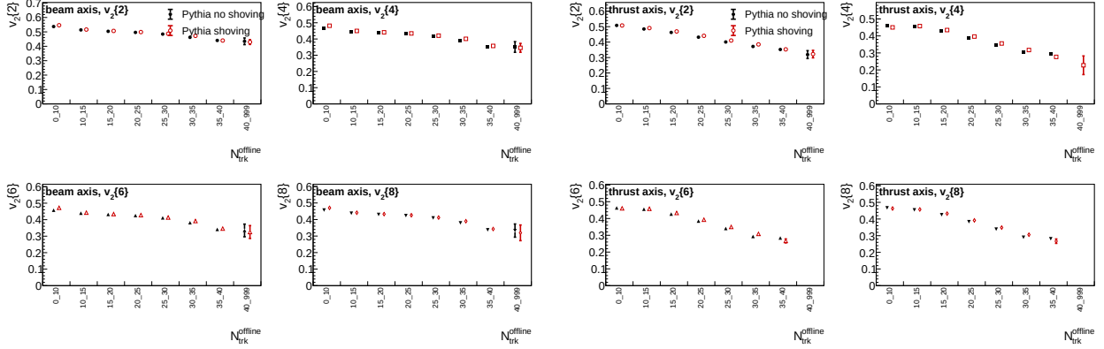
Figure 31: Generator-level Pythia no-shoving/shoving comparison for Event-shape selection S > 0.12 . Left: beam axis. Right: thrust axis.
