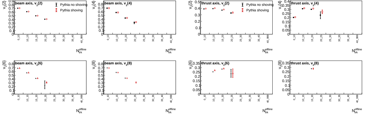
Figure 28: Generator-level Pythia no-shoving/shoving comparison for Negative charged particles only. Left: beam axis. Right: thrust axis.
