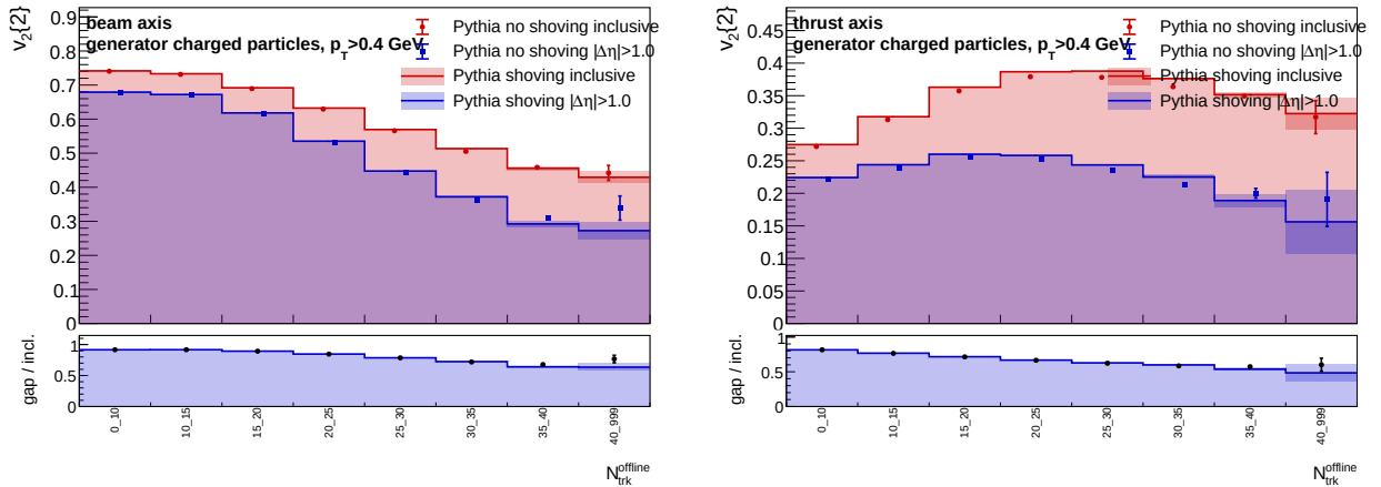
Figure 15: Generator-level Pythia no-shoving/shoving comparison for Two-particle rapidity-gap selection |\Delta\eta| > 1.0 . Left: beam axis. Right: thrust axis.
