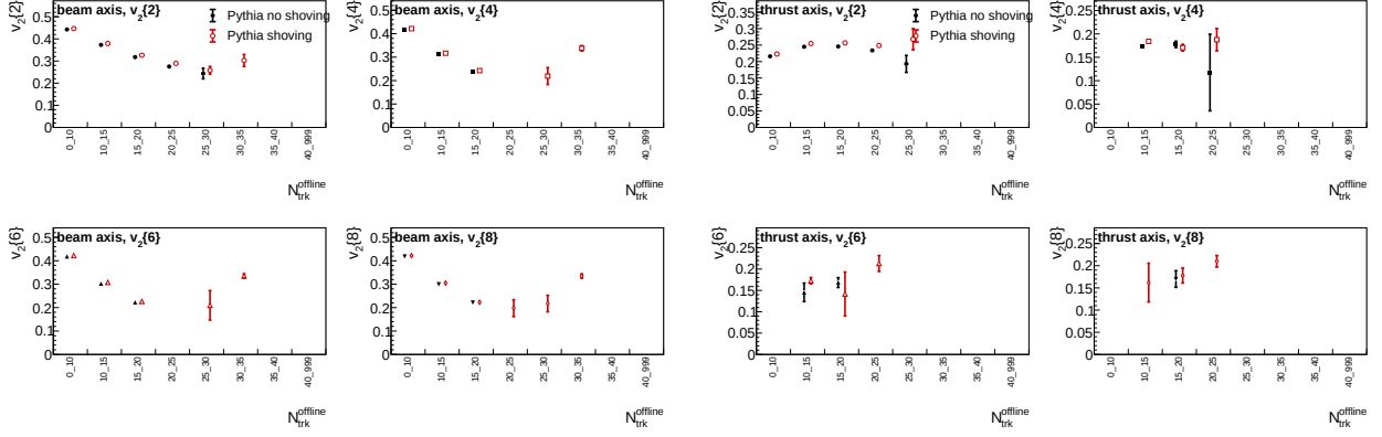
Figure 24: Generator-level Pythia no-shoving/shoving comparison for Track selection 0.4 < p_T < 1 GeV. Left: beam axis. Right: thrust axis.
