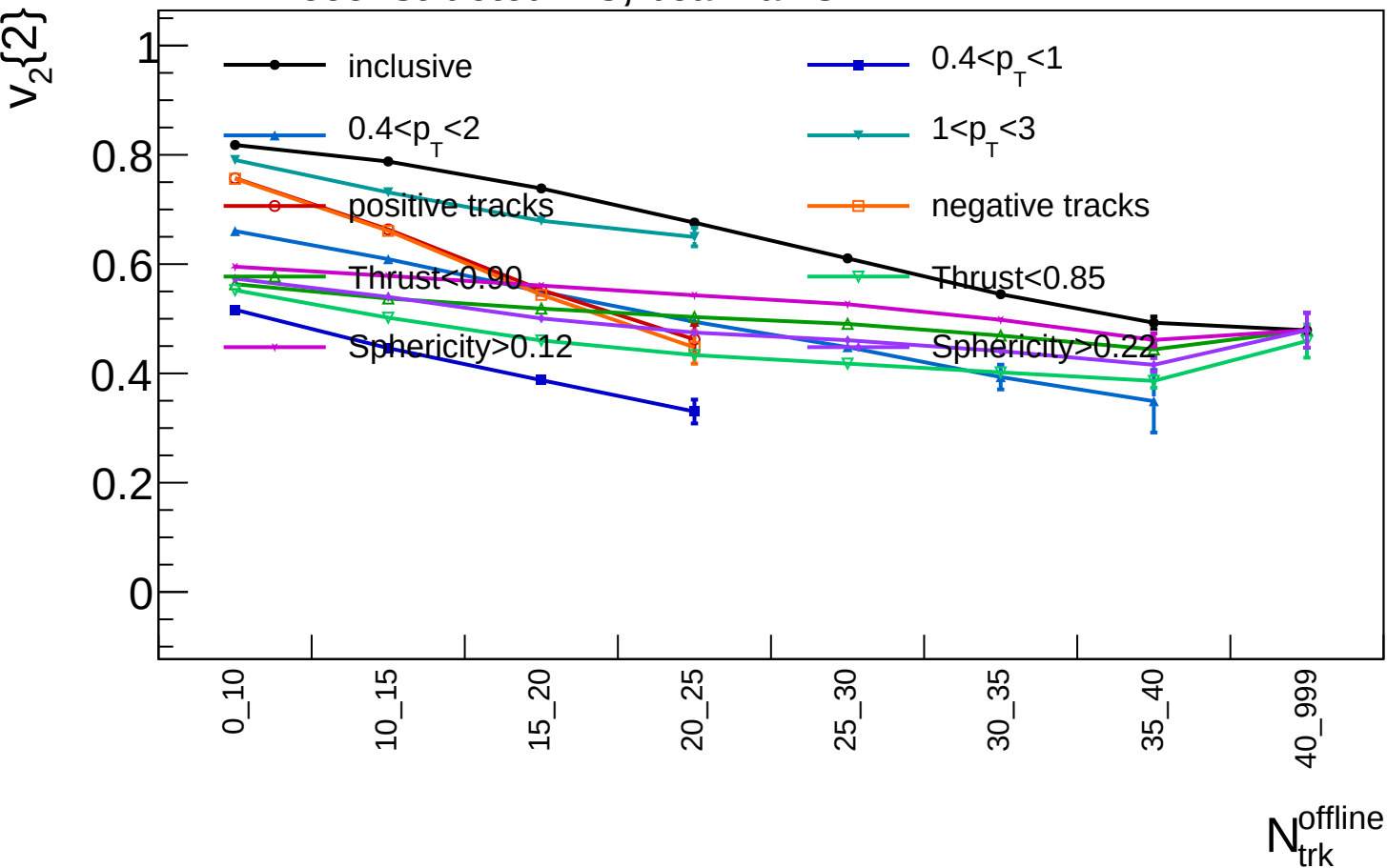
LEP1 reconstructed MC, beam axis
